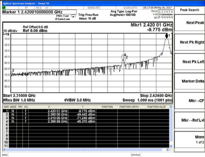
2420 MHz – Peak
