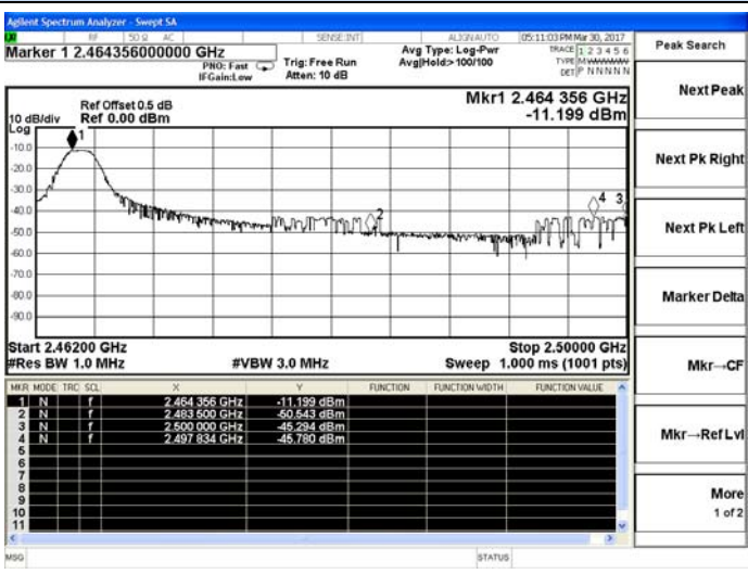
2465 MHz – Peak
