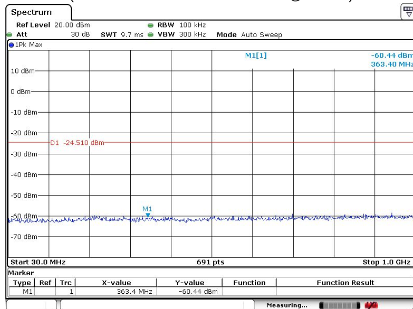
(Plot 4.9.2 A1: Channel 00: 2402MHz @ 8DPSK)
