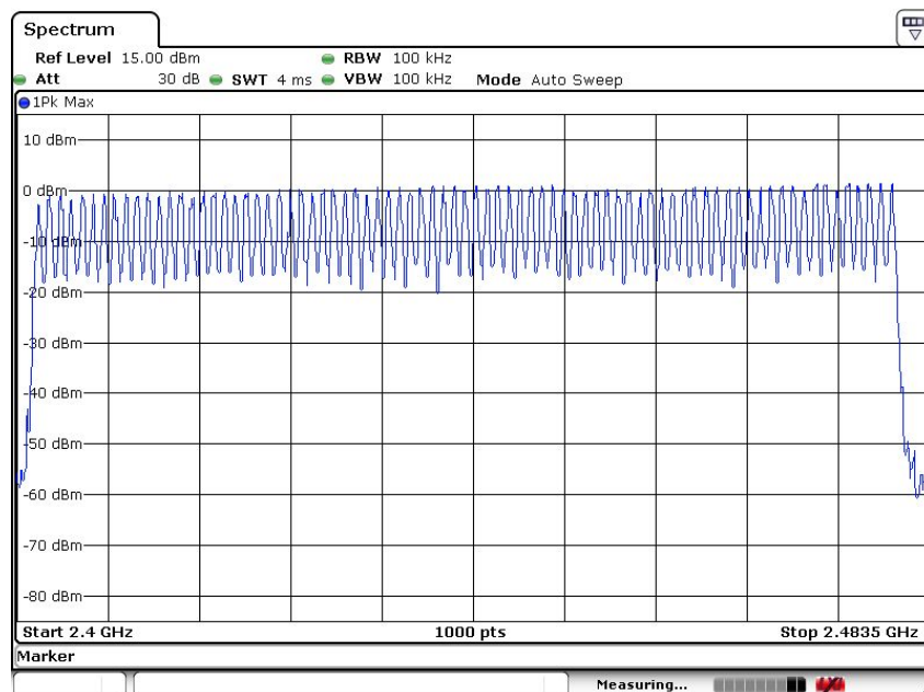
(Plot 4.7.1 A1: @ GFSK)
