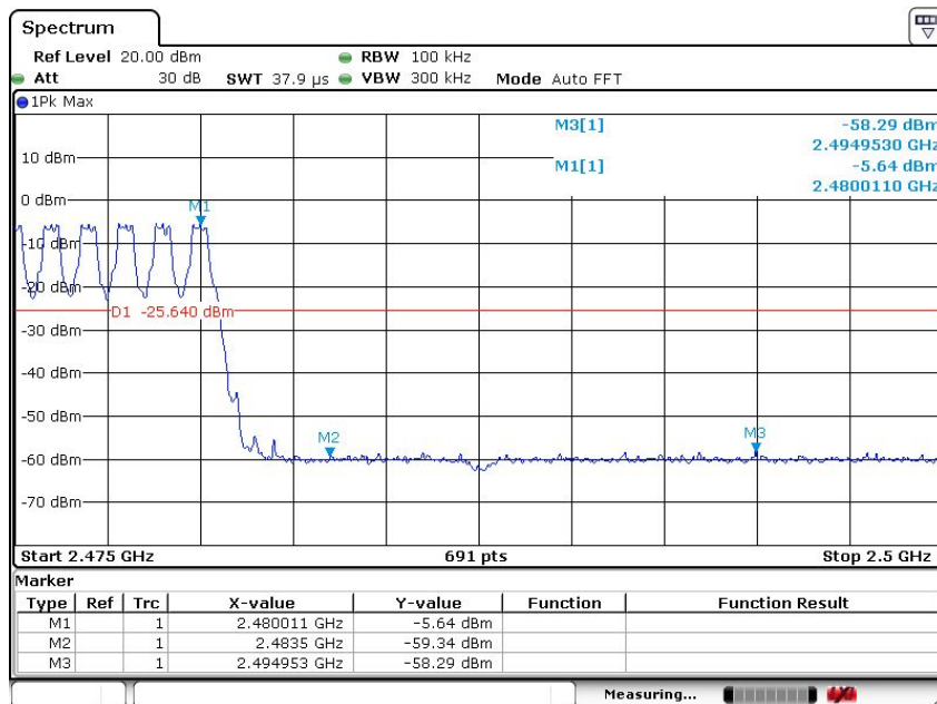
(Plot 4.5.2.1 B: Hopping Mode @ GFSK)
