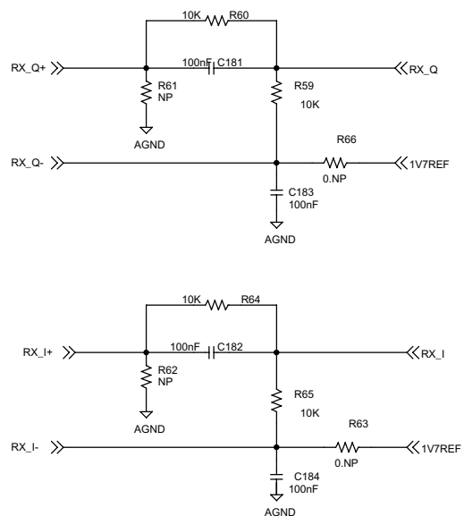
RX I & Q +/- INTERFACE
