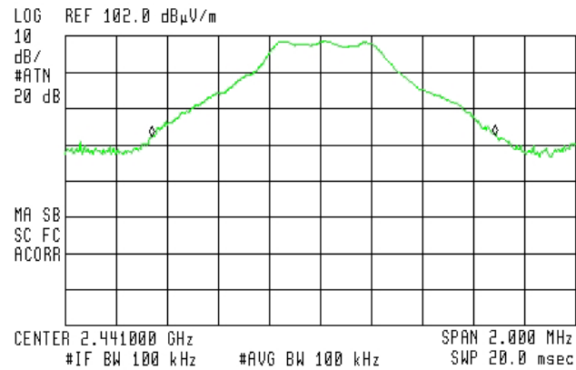
Figure 21 — 2441.0 MHz
