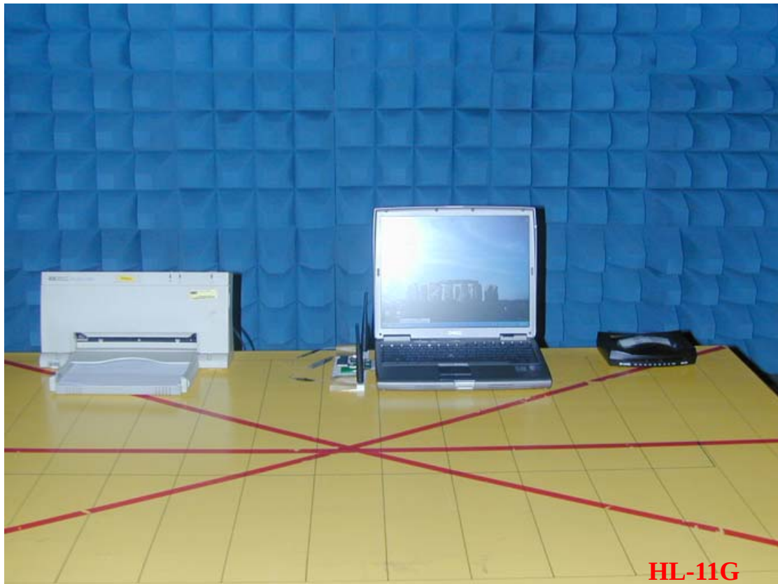
Photo 1: Radiated Emission Test Set-up
