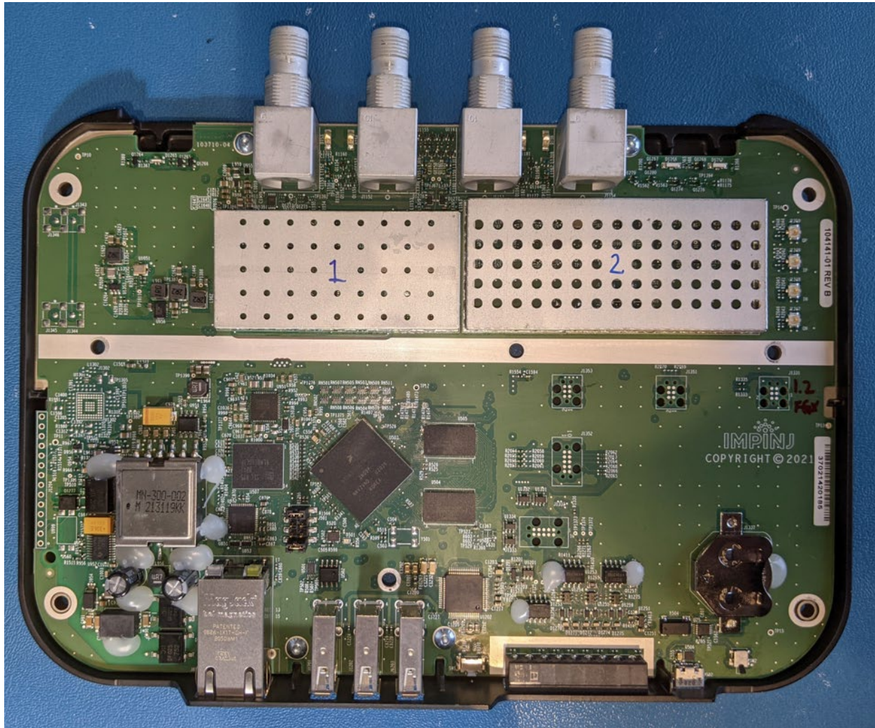
Figure 7: Top Internal View of IPJ-R510 in metal enclosure
