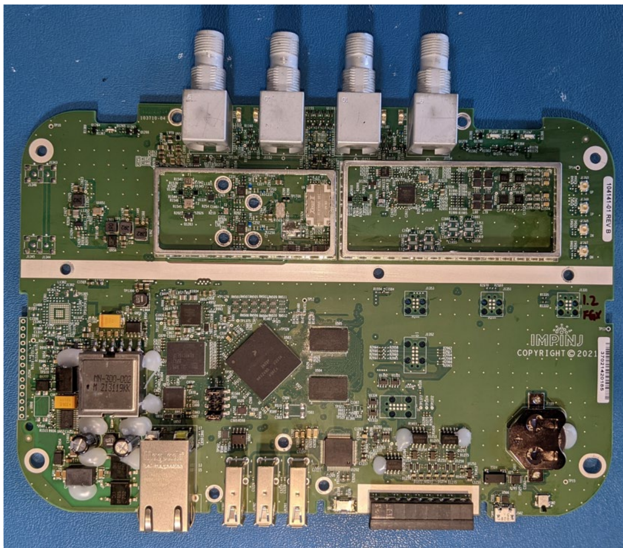
Figure 9: Top Internal View of IPJ-R510
