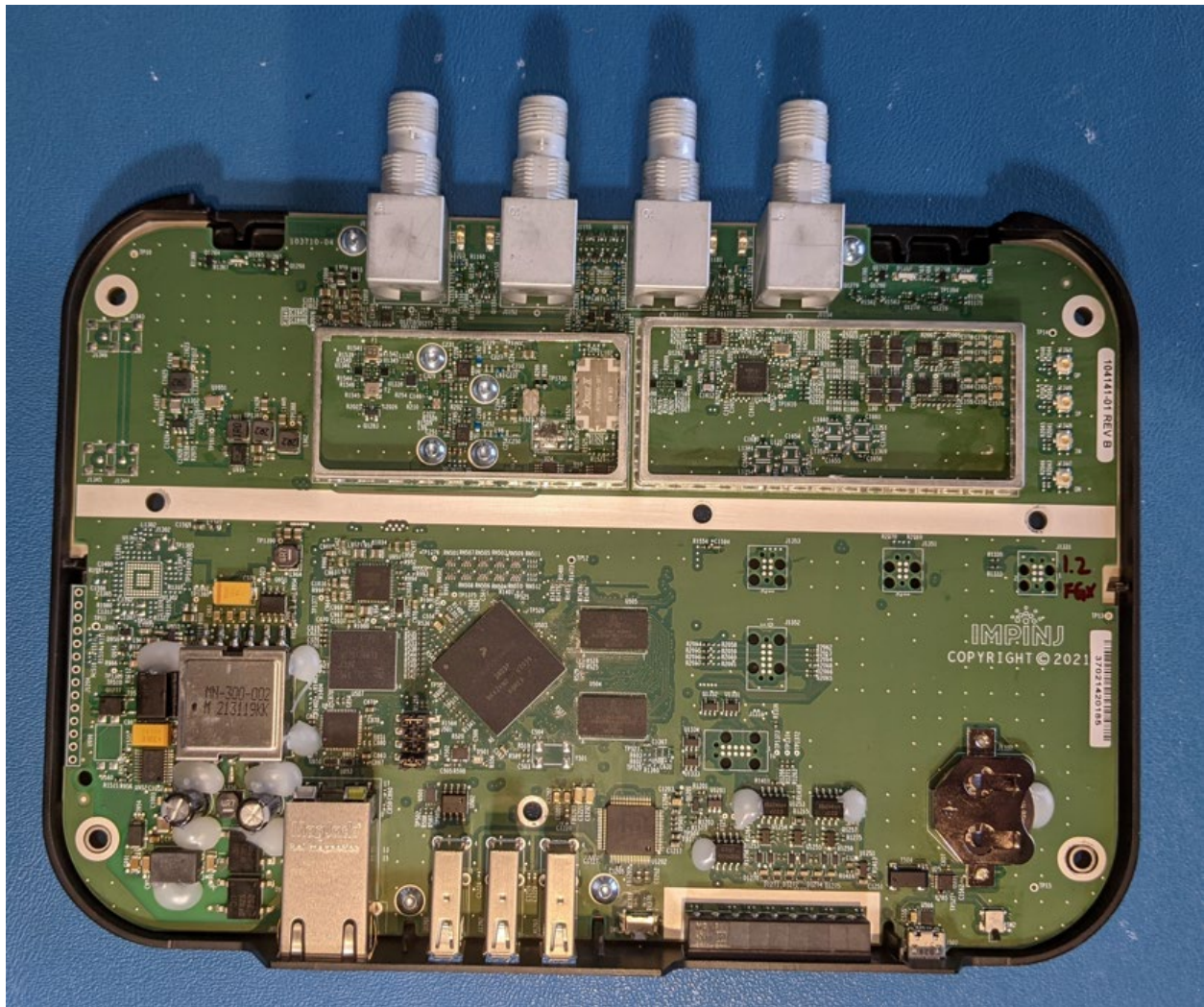
Figure 8: Top Internal Photo of IPJ-R510 without Shields
