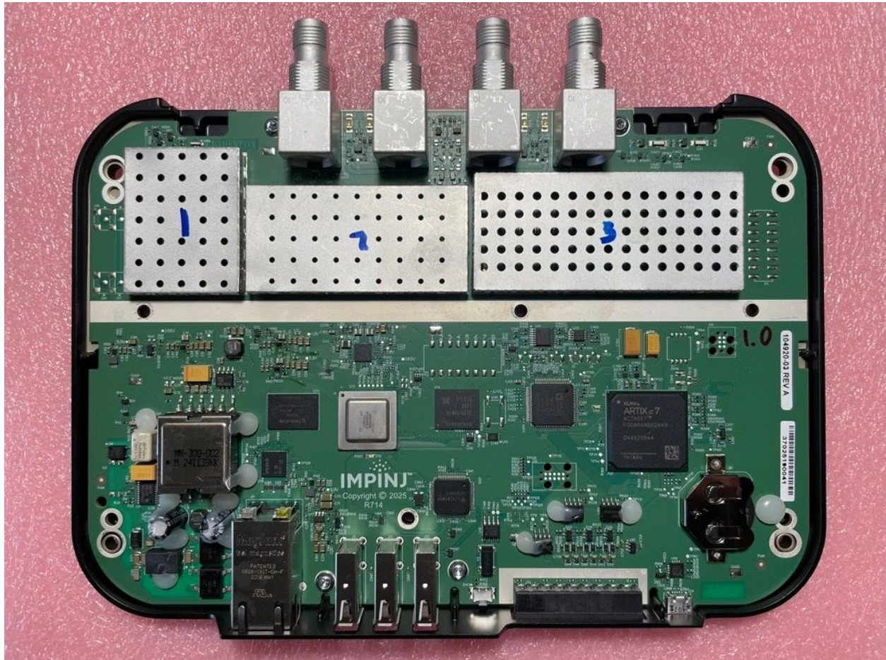
Figure 7: Top Internal View of IPJ-R700 in metal enclosure
