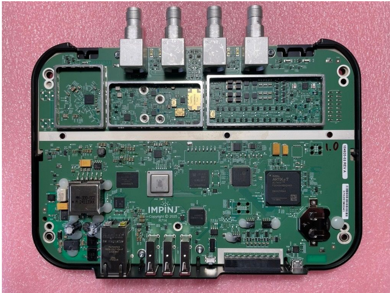
Figure 8: Top Internal Photo of IPJ-R700 without Shields
