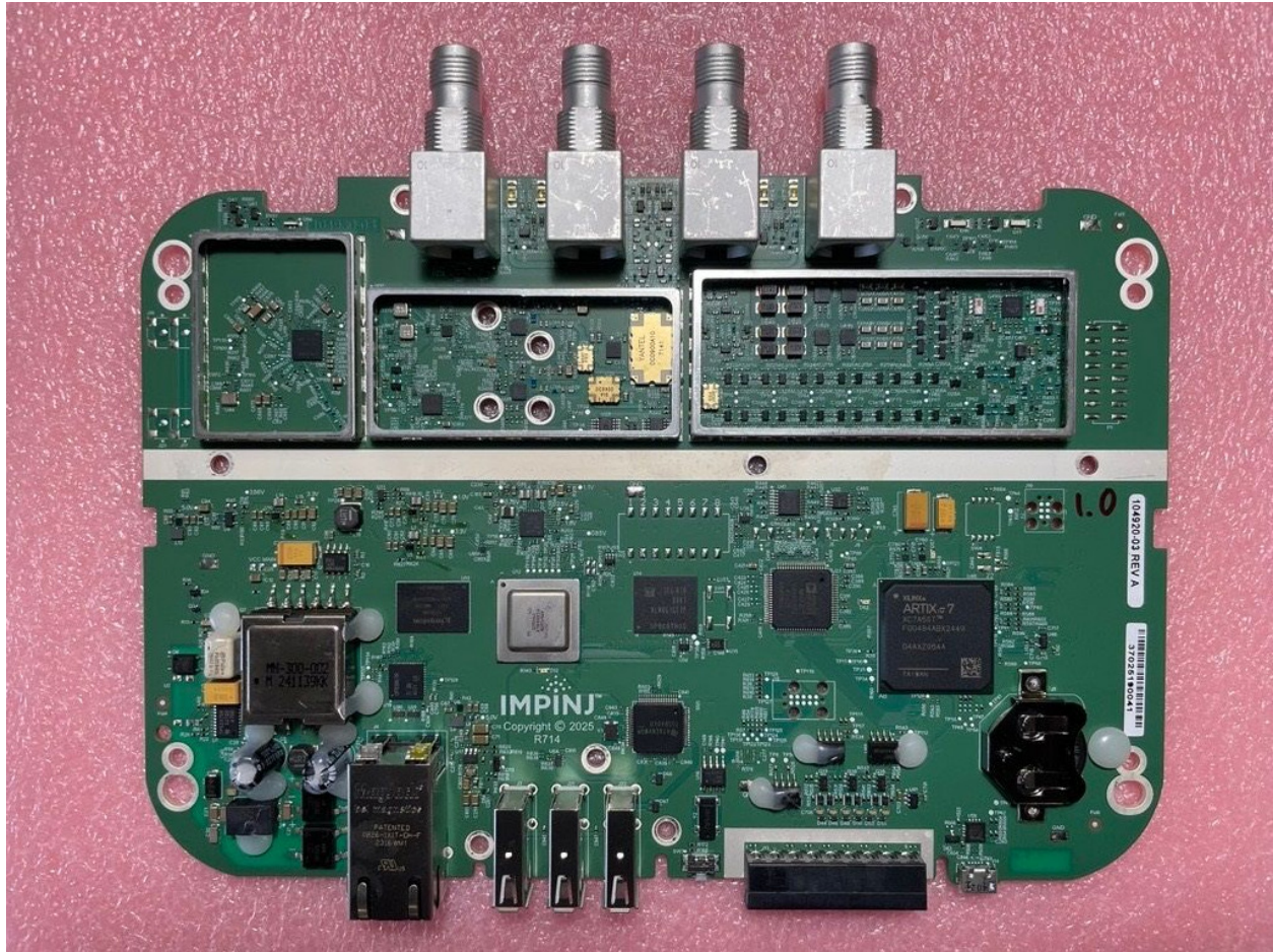
Figure 9: Top Internal View of IPJ-R700
