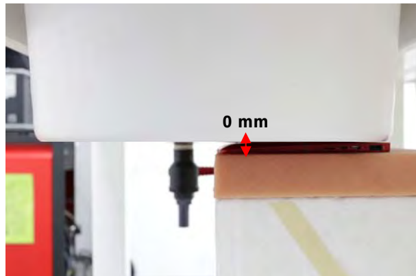
Fig.3 Back side to flat phantom
