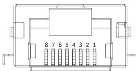
▲ Figure B.5 LAN RJ-45 Connector
