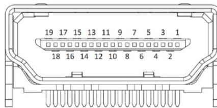
▲ Figure B.3 HDMI Connector
