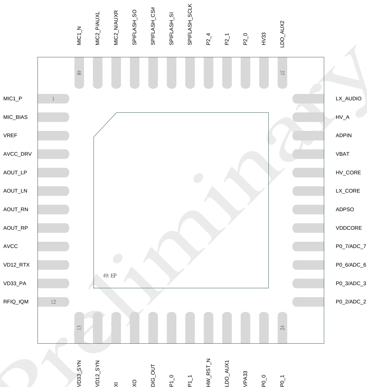
Figure 6. PIN OUT (TOP View) RTL8763BS QFN48
