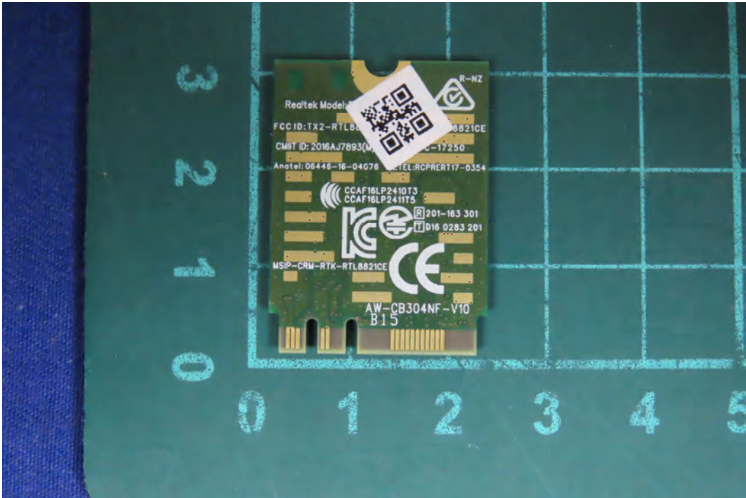
(24) EUT Photo_RTL8821CE
