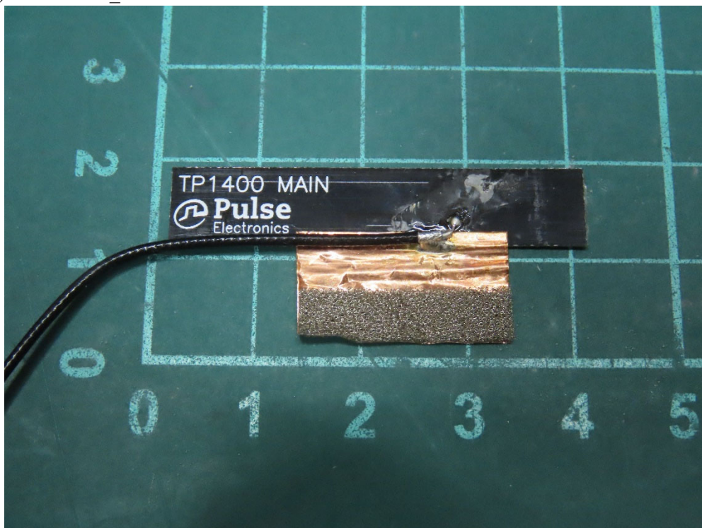
(31) EUT Photo_Pulse Main Antenna
