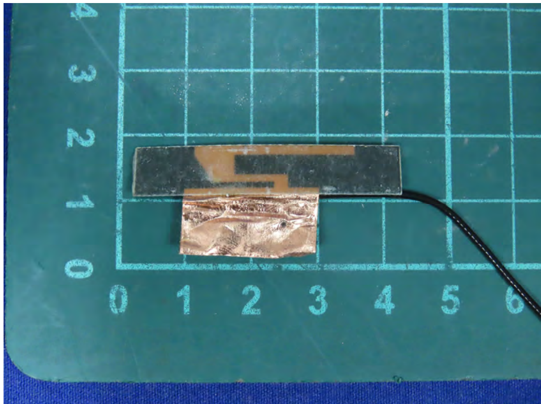
(34) EUT Photo
