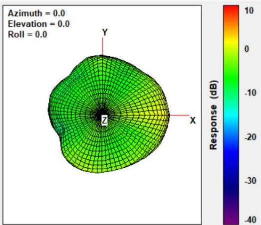
Radiation Pattern of WLAN Antenna (5925MHz)
