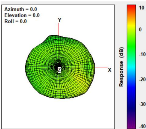
Radiation Pattern of WLAN Antenna (5350MHz)
