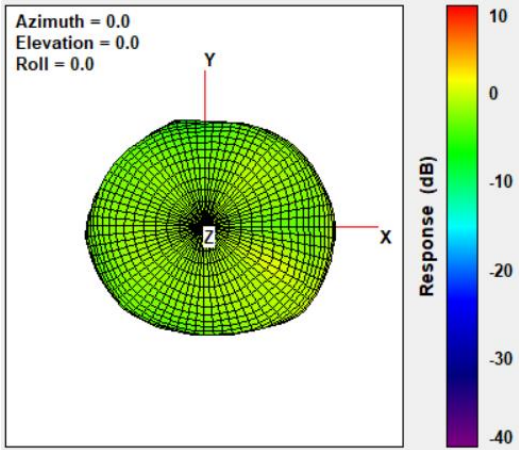
Radiation Pattern of WLAN Antenna (5250MHz)
