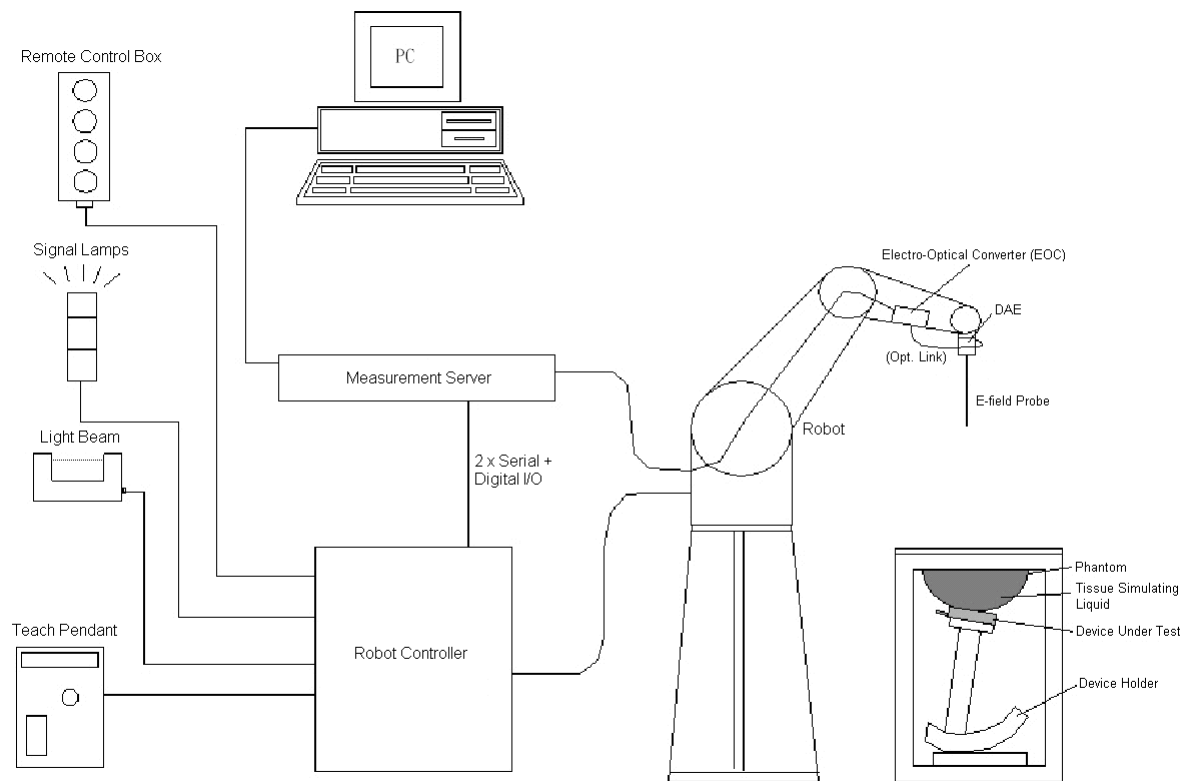
Fig-3.1 SPEAG DASY52 System Setup
