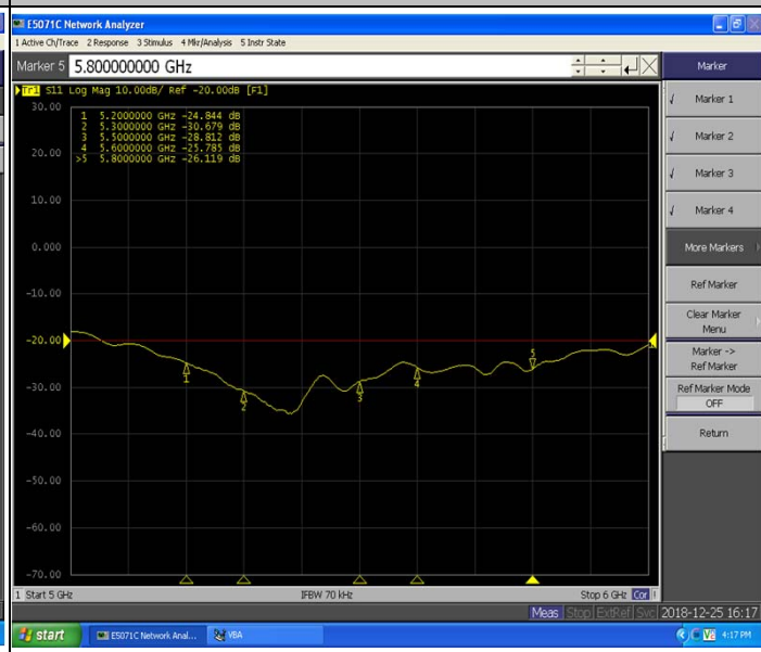
Return Loss-Head
