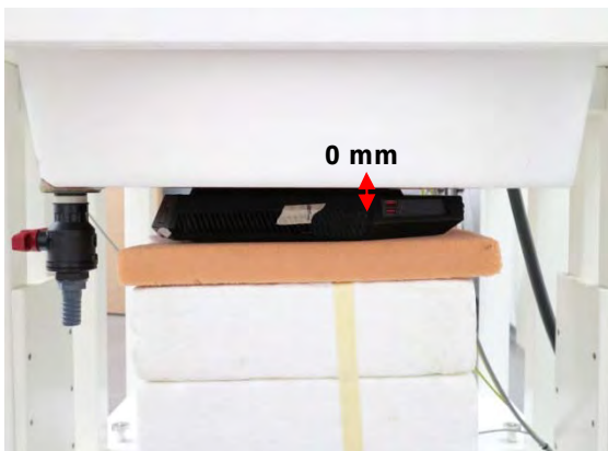
Fig.14 EUT position(3-1) to flat phantom
