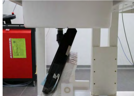
Fig.12 EUT position(2-7) to flat phantom
