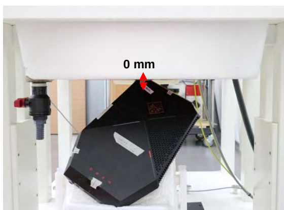
Fig.8 EUT position(2-3) to flat phantom
