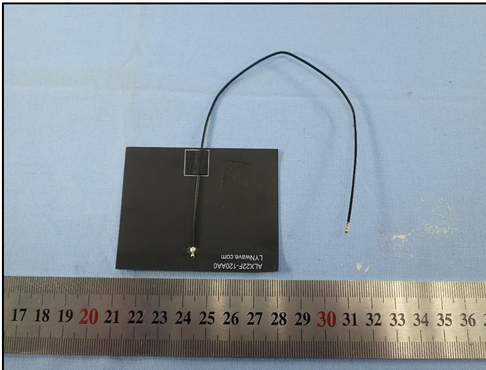
Antenna NO. 3 (Monopole) (Brand: LYNwave, Model: ALX22F-120AA0-00)
