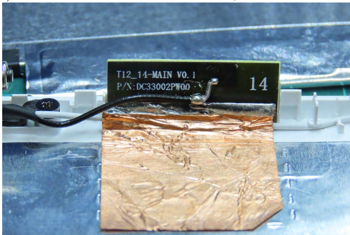
(24) EUT Photo - Antenna: SOUTHSTAR TECHNOLOGY CO.,LTD
