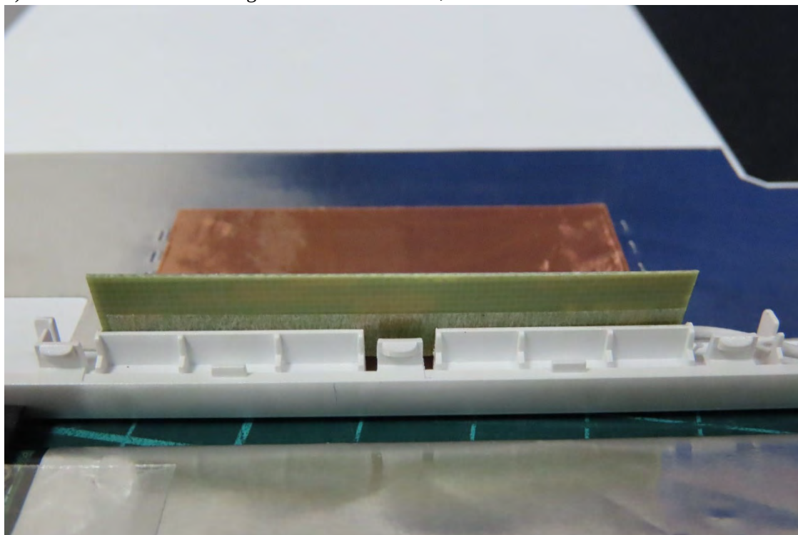
(31) EUT Photo - Antenna: High-Tek Electronics Co., Ltd.
