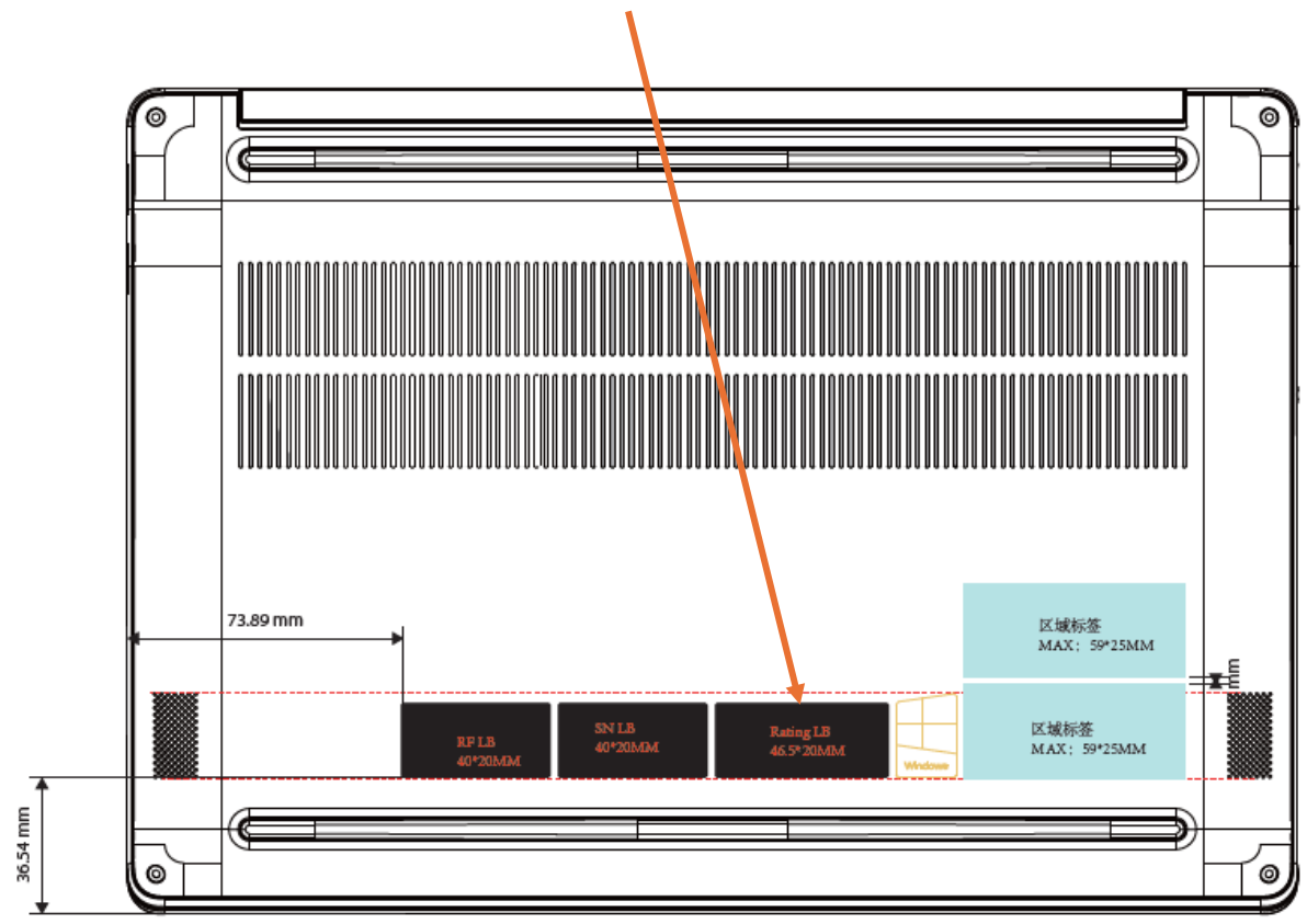
Rating label
