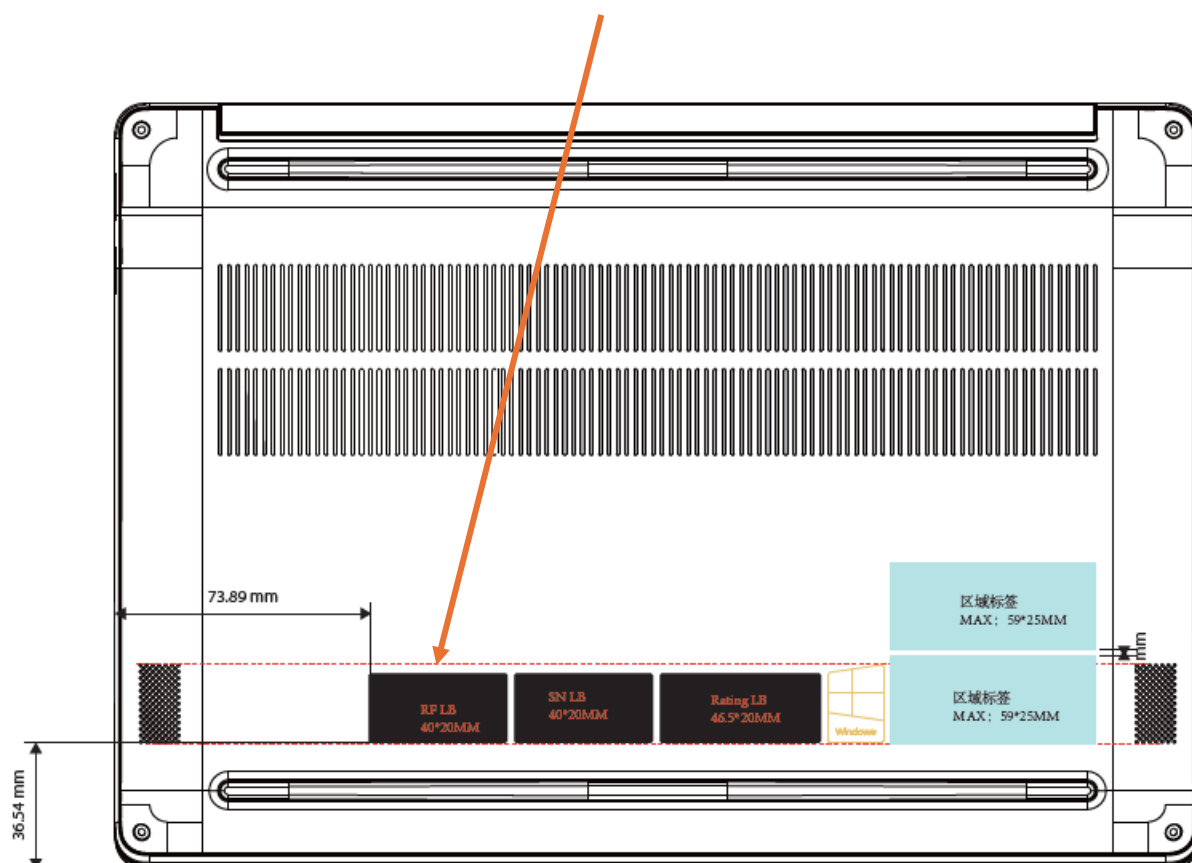
RF Label
