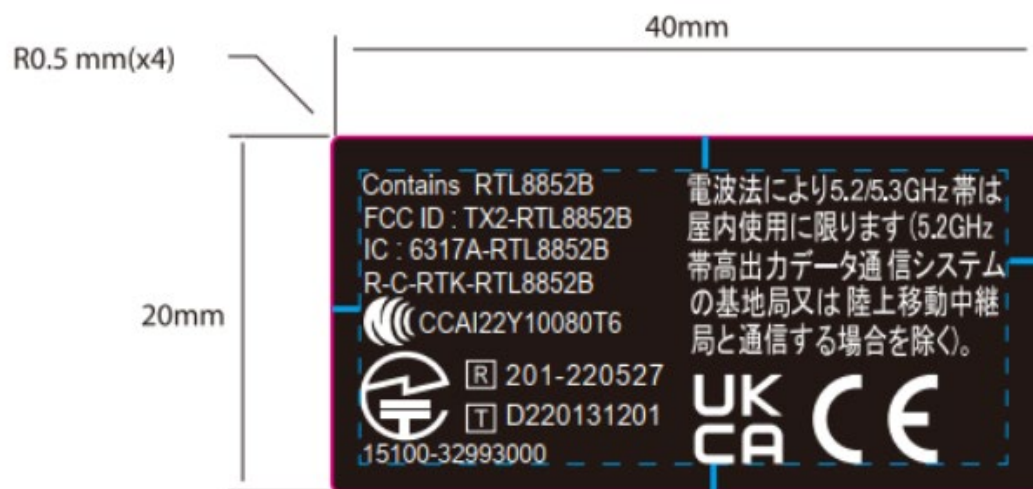
RF Label
