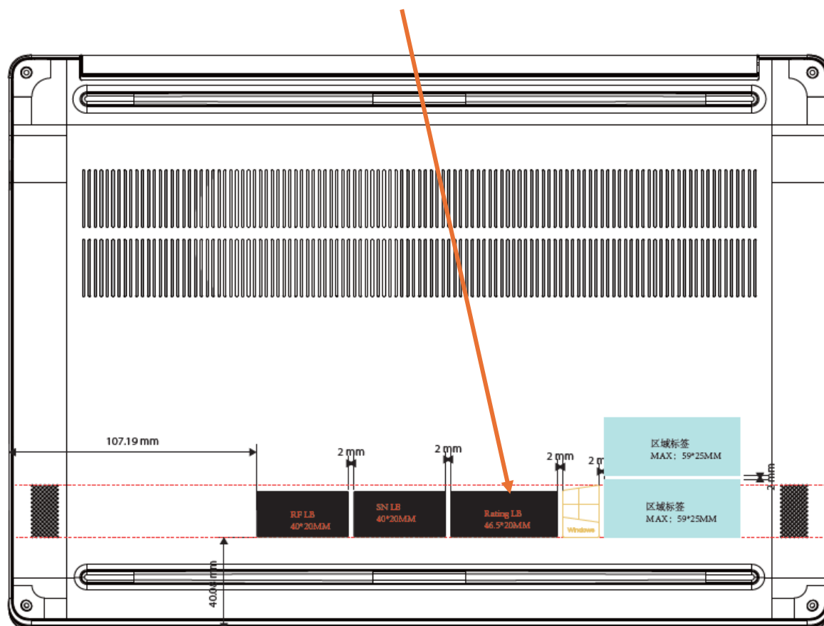
Rating label
