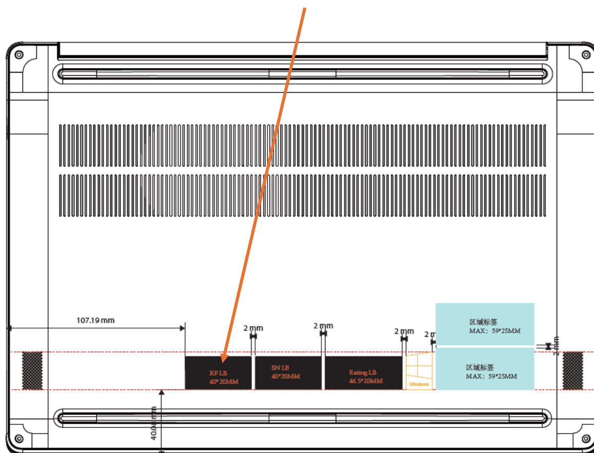
RF Lable
