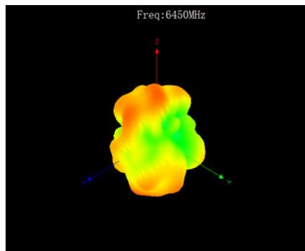
Max Antenna 3D Radiation Pattern 6525-6875 MHz
