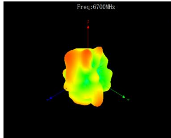
Max Antenna 3D Radiation Pattern 6875-7125 MHz
