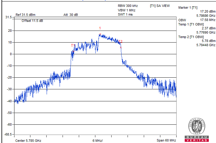
802.11ax (RU106) / Chain1: CH 157
