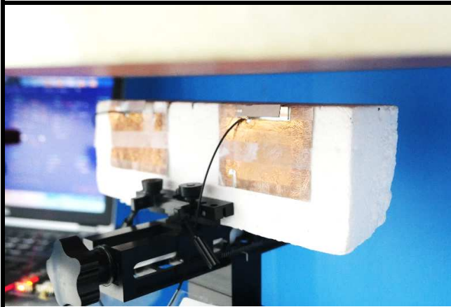
Top Side of EUT Tested at 11 mm
