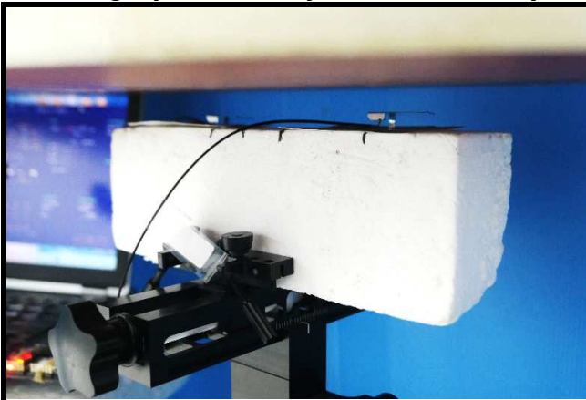
Front Face of EUT Tested at 11 mm
