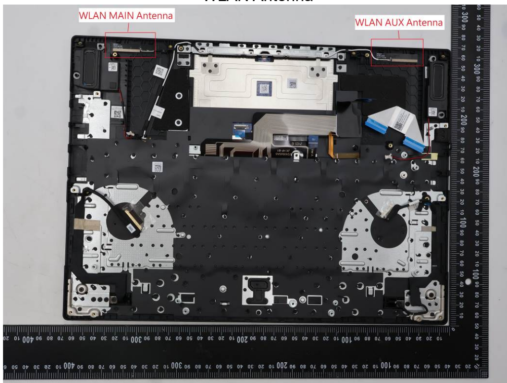
WLAN Antenna
