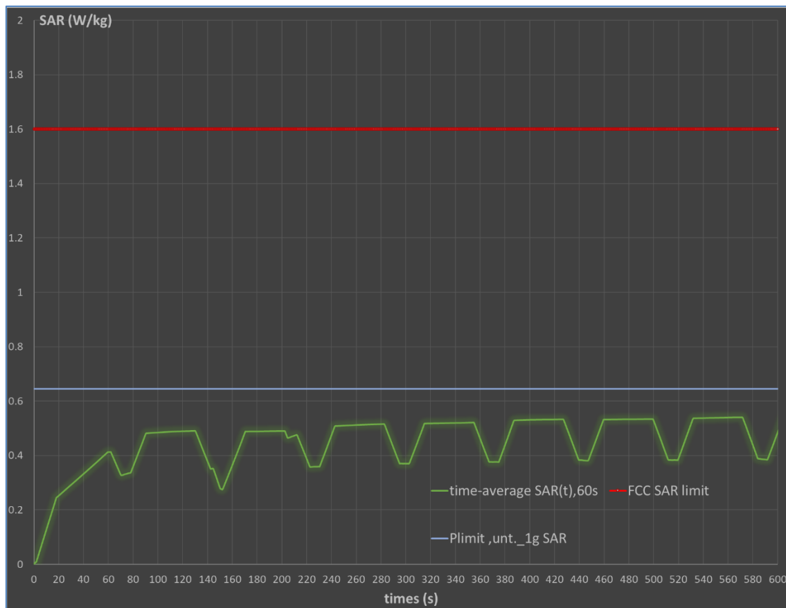
Figure 7-2: Time-Averaged SAR Measurement Result for Test Scenario 3
