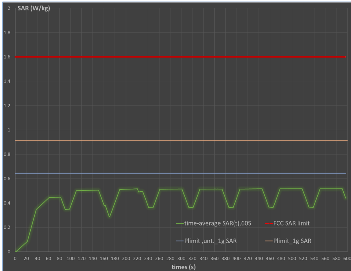
Figure 6-3: Time-Averaged SAR Over Time for Test Scenario 1
