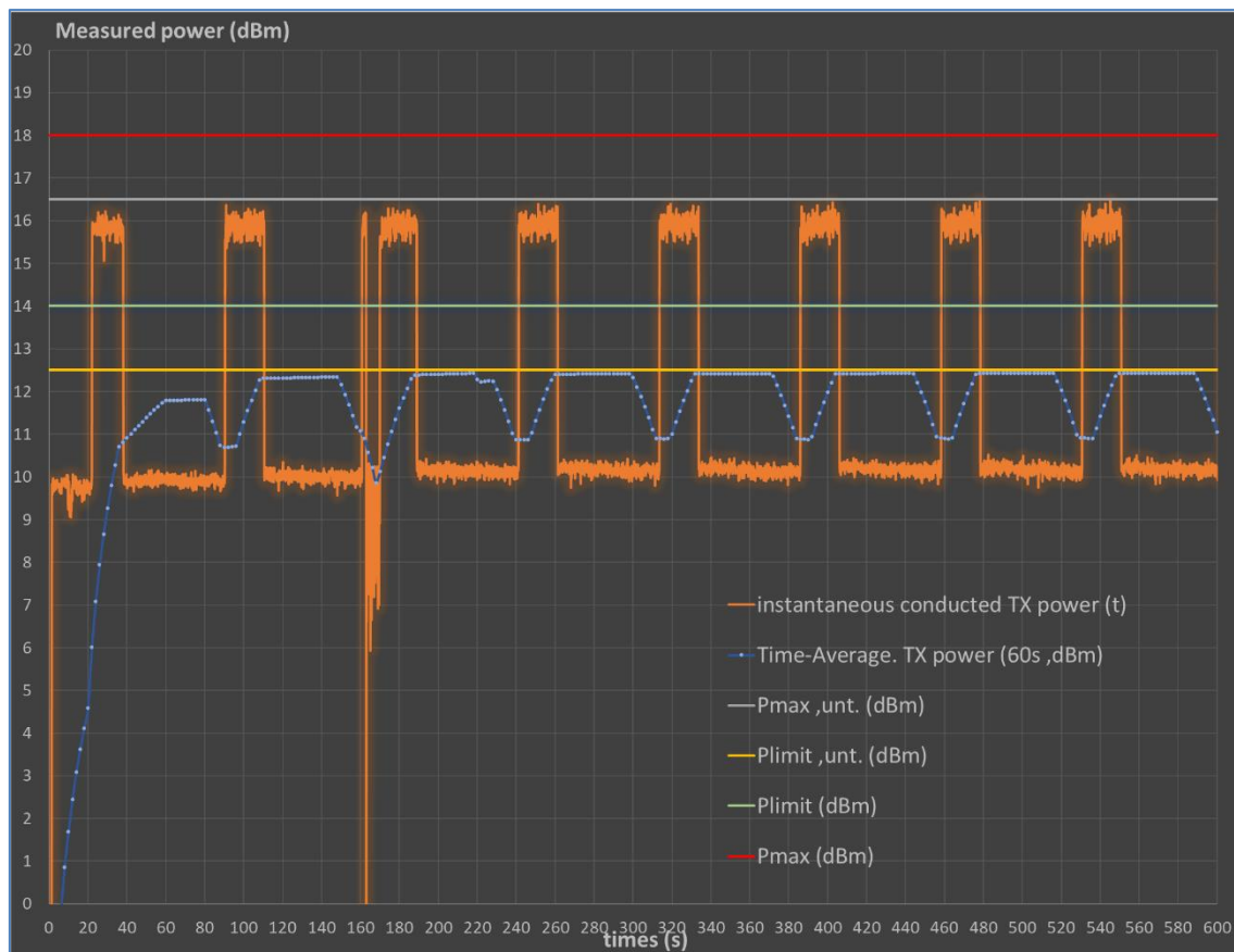
Figure 6-2: Time-Averaged Conducted Tx Power Over Time for Test Scenario 1
