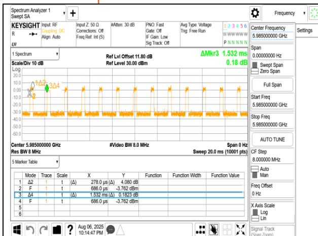
802.11ax_80MHz_Chain0_5985MHz
