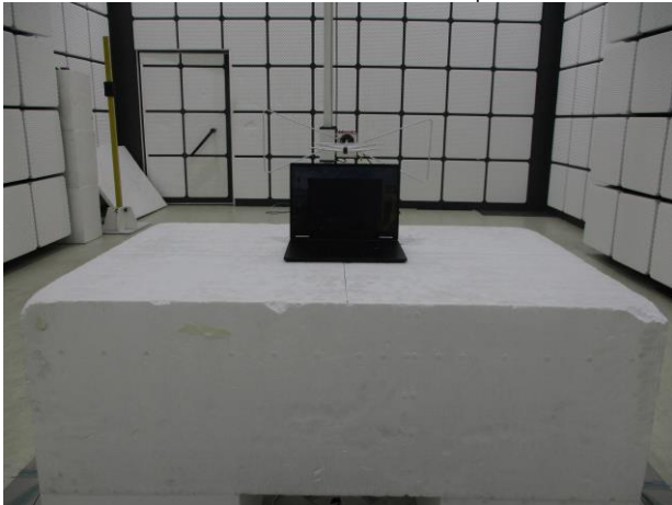
FCC_15_407_Radiated_Setup
