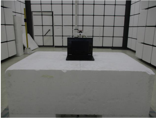
FCC_15_407_6E_Radiated_Setup
