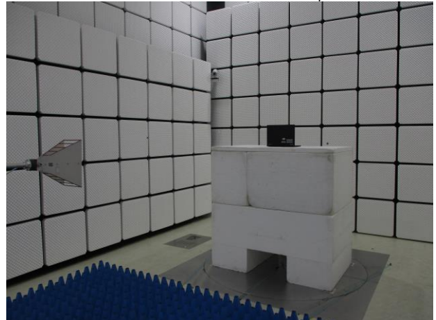
FCC_15_407_6E_Radiated_Setup
