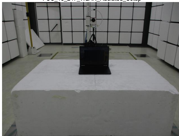
FCC_15_247_WLAN_Radiated_Setup
