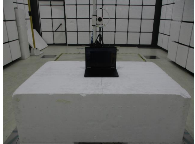
FCC_15_407_6E_Radiated_Setup
