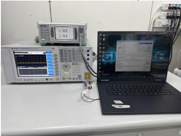
FCC_15_247_BLE_Conducted_Setup
