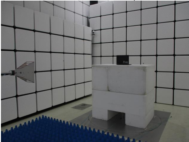
FCC_15_407_Radiated_Setup
