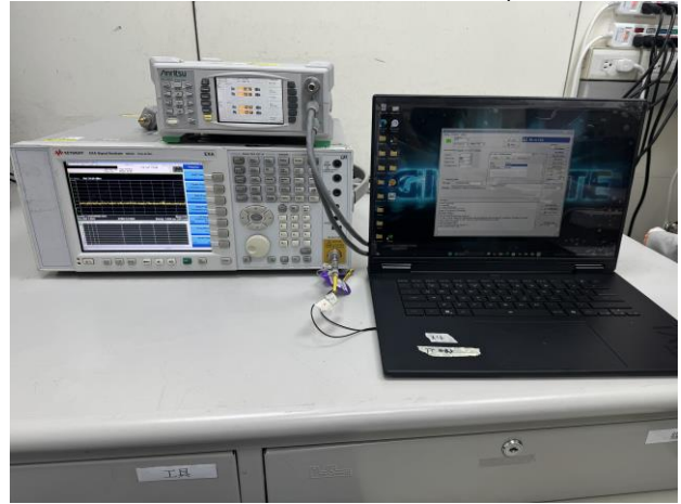
FCC_15_247_WLAN_Conducted_Setup
