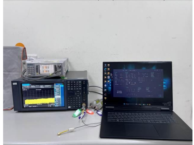
FCC_Part 15.407_WLAN(5G)_Conducted_Setup
