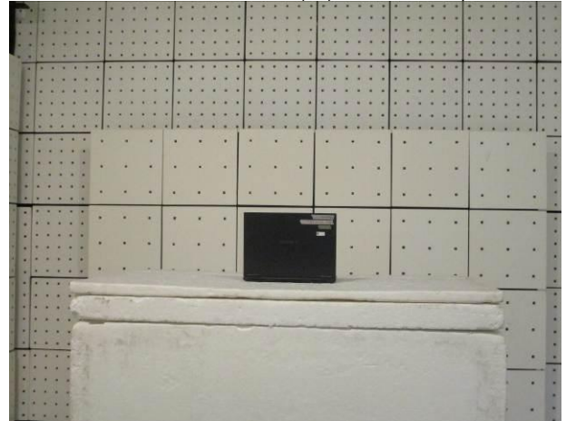
FCC_Part 15.407_WLAN(6E)_Radiated_Setup
