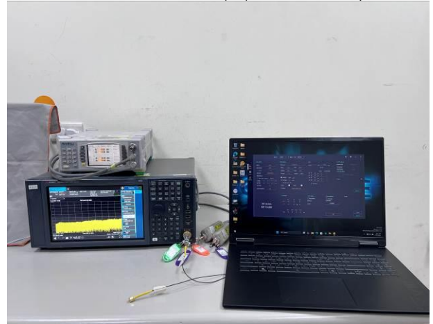
FCC_Part 15.407_WLAN(6E)_Radiated_Setup
