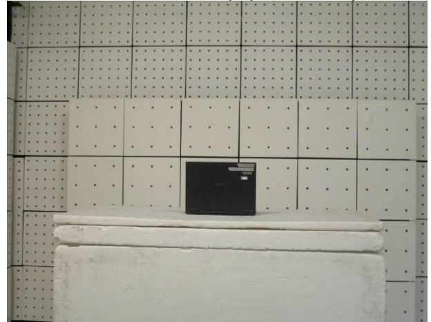
FCC_Part 15.407_WLAN(5G)_Radiated_Setup
