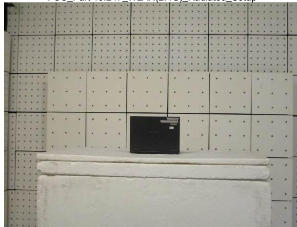
FCC_Part 15.247_WLAN(2.4G)_Radiated_Setup
