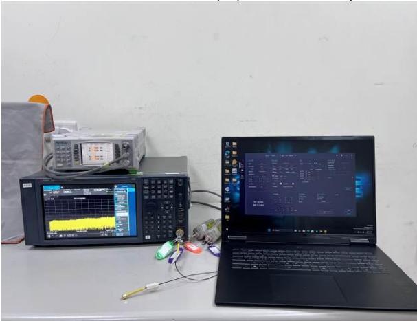
FCC_Part 15.247_BLE_Conducted_Setup
