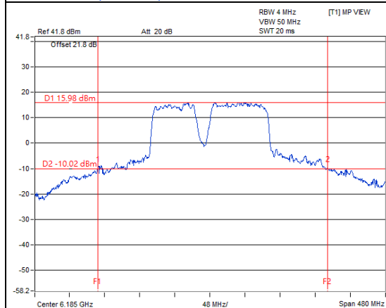
802.11be (EHT160) 996+484+242-tone MRU / Chain 1: CH 47
