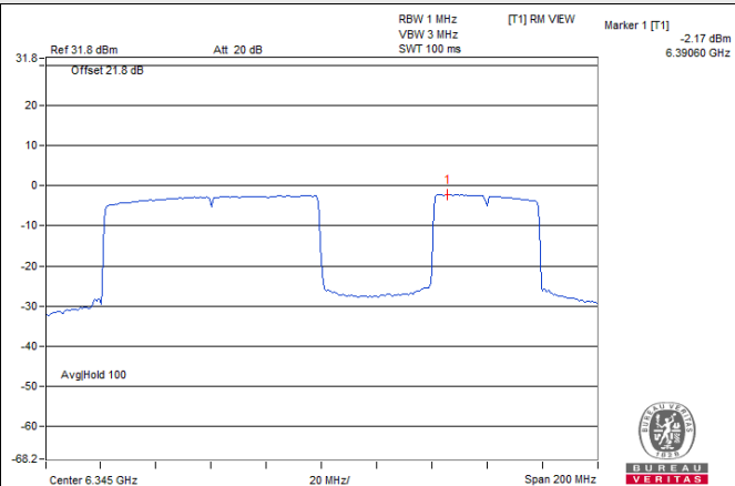
802.11be (EHT160) 996+484-tone MRU / Chain 1: CH 79
