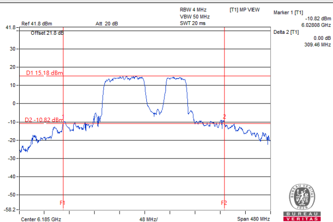
802.11be (EHT160) 996+484-tone MRU / Chain 1: CH 47
