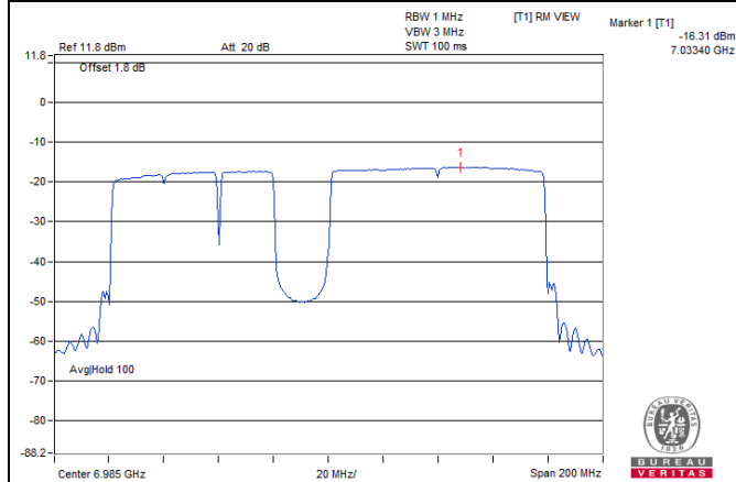
802.11be (EHT160) 996+484+242-tone MRU / Chain 1: CH 207
