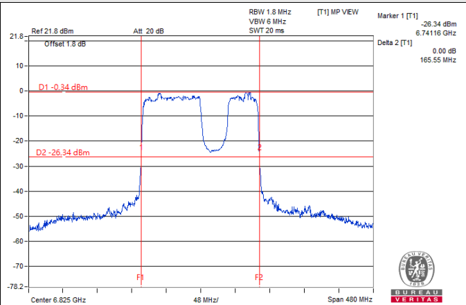
802.11be (EHT160) 996+484-tone MRU / Chain 1: CH 175
