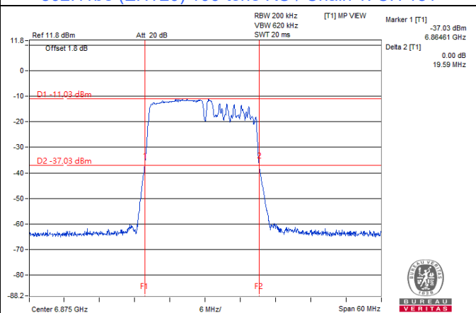
802.11be (EHT20) 106+26-tone MRU / Chain 1: CH 185
