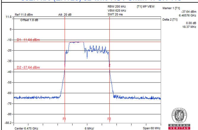
802.11be (EHT20) 52+26-tone MRU / Chain 1: CH 105
