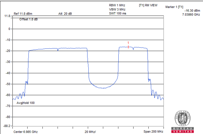
802.11be (EHT160) 996+484-tone MRU / Chain 1: CH 207
