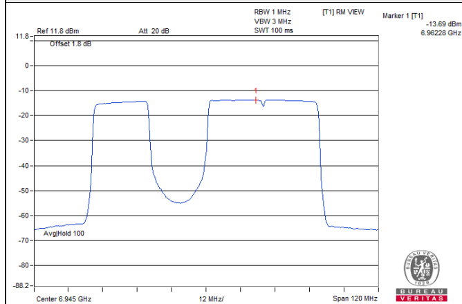
802.11be (EHT80) 484+242-tone MRU / Chain 1: CH 199
