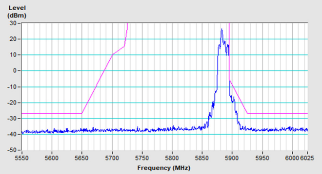
Vertical (Peak)
