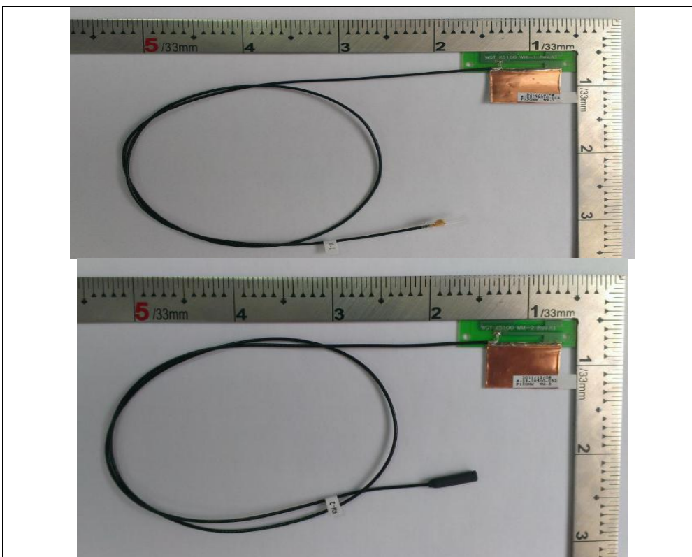
Antenna 38: Brand: WGT / Model: SKX51WMPB01+C (WM1) & SKX51WMPB02+C (WM2)
