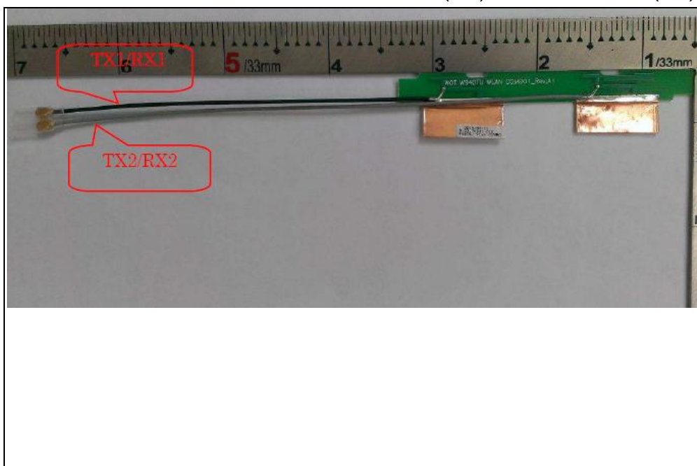
Antenna 30: Brand: WGT / Model: SK94SWMPB01+B (TX1) 7 SK94SWMPB01+B (TX2)
