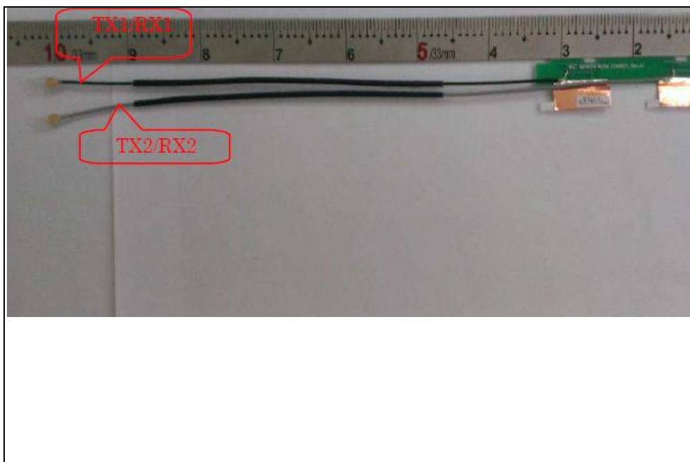
Antenna 31: Brand: WGT / Model: SK94TWMPB01+B (TX1) & SK94TWMPB01+B (TX2)
