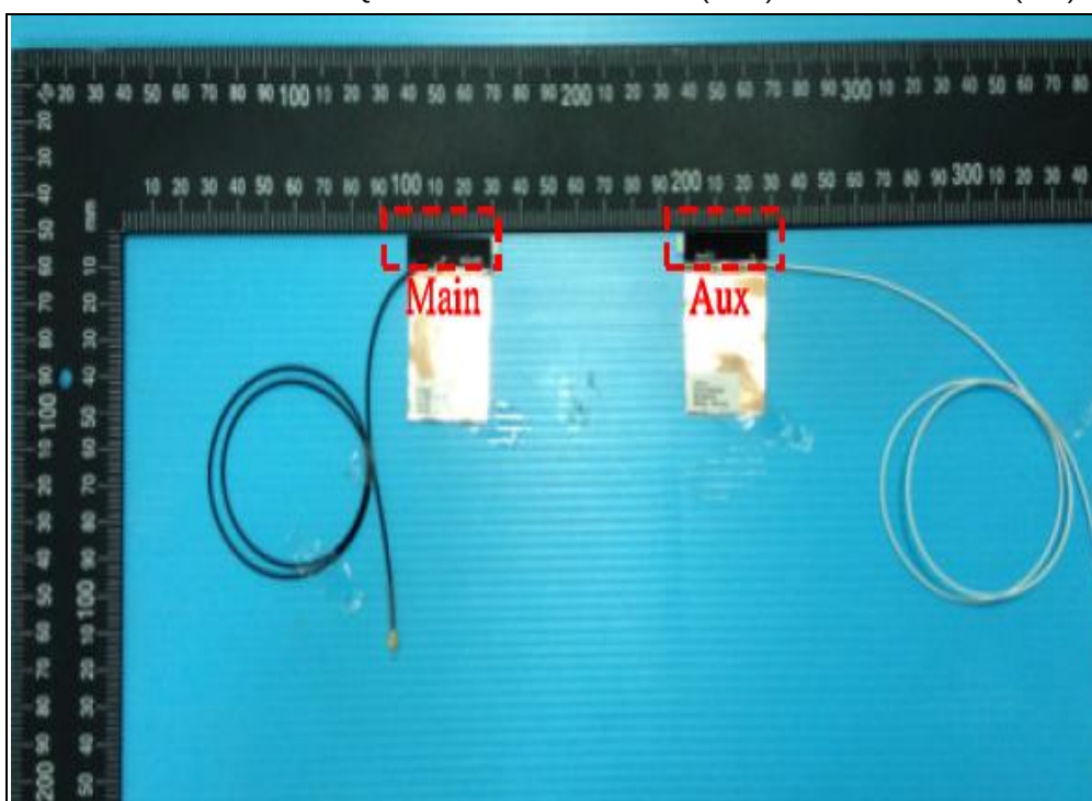
Antenna 39: Brand: INPAQ / Model: WA-P-LB-02-122 (Main) & WA-P-LB-01-072 (Aux)
