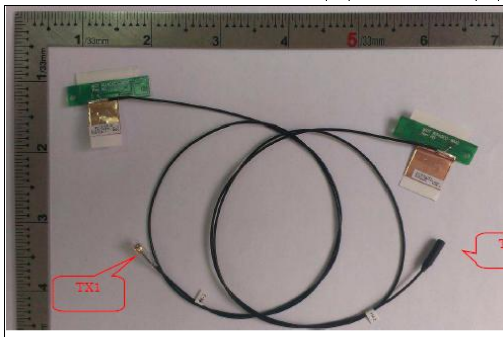
Antenna 24: Brand: WGT / Model: SK547WMPB01+A (Tx1) & SK549WMPB02+A (Tx2)
