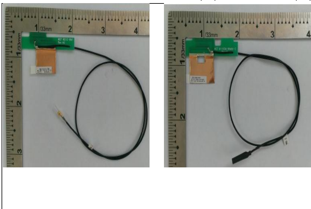
Antenna 16: Brand: WGT / Model: SKM11WMPB03+A (Tx1) & SKM11WMPB02+D (Tx2)
