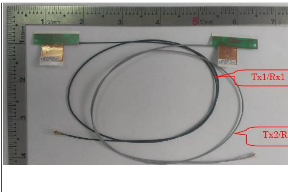
Antenna 25: Brand: WGT / Model: SK555WMPB01+B (Tx1) & SK555WMPB02+B (Tx2)
