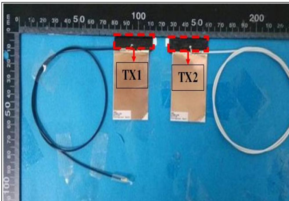
Antenna 40: Brand: Smart Approach / Model: SE-ECZ50-001 (Tx1) & SE-ECZ50-002 (Tx2)
