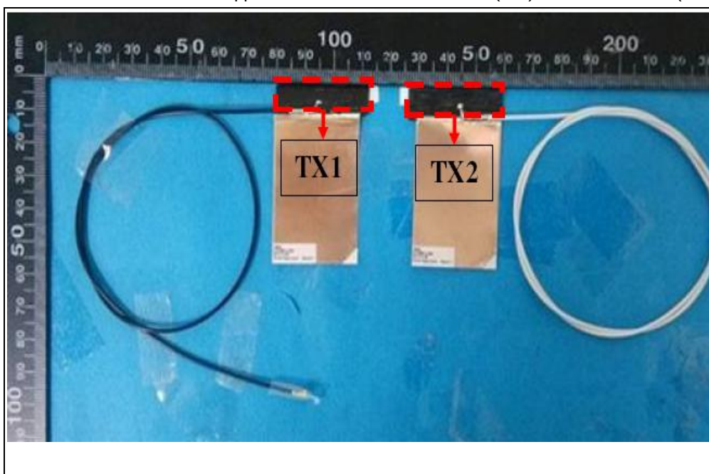
Antenna 42: Brand: Smart Approach / Model: SE-ECZ70-001 (Tx1) & SE-ECZ70-002 (Tx2)
