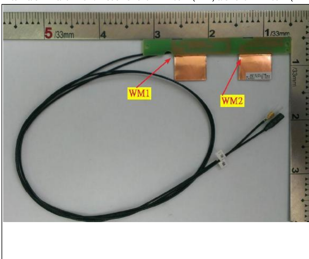
Antenna 34: Brand: WGT / Model: SKC45WMPB03+B (WM1) & SKC45WMPB03+B (WM2)
