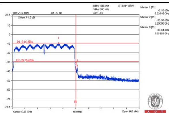
EUT (Client ) links with master on 11AC VHT80 mode
