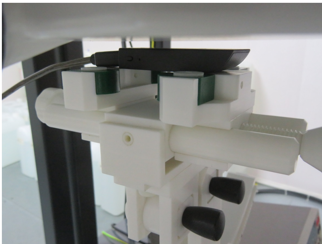
5mm body Horizontal-Down Side Setup Photo – Test Position 2
