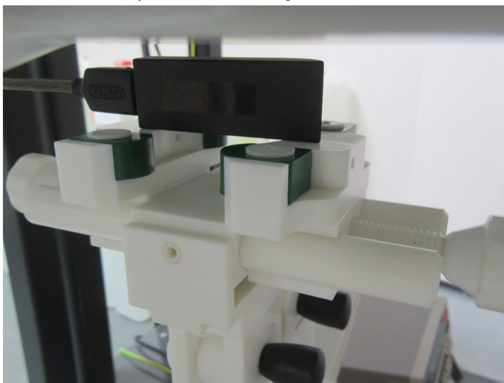
5mm body Vertical-Back Side Setup Photo – Test Position 4
