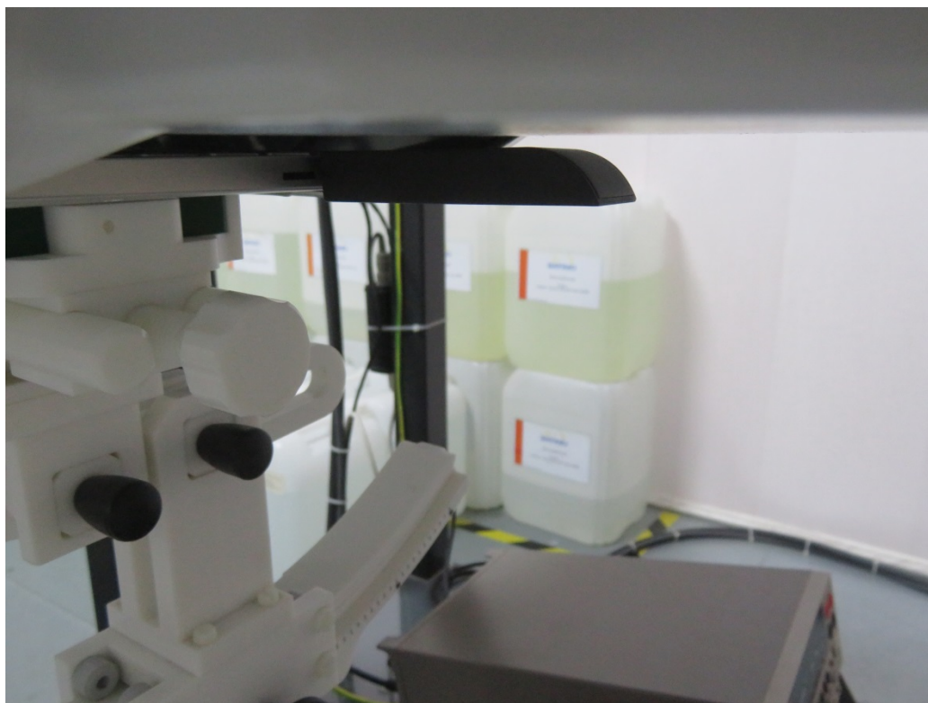
5mm body Horizontal-Up Side Setup Photo – Test Position 1
