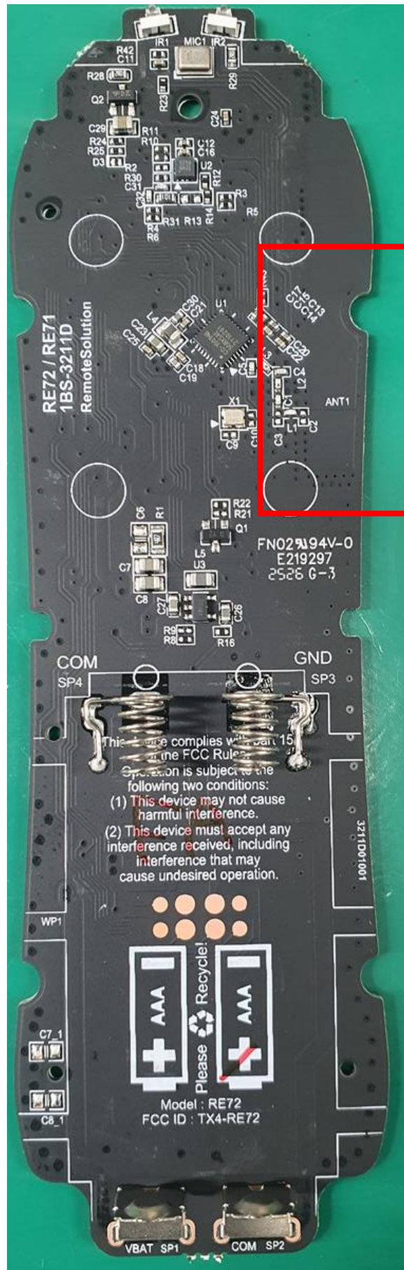
PCB Antenna
