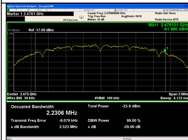
20dB Bandwidth – High CH 2475
