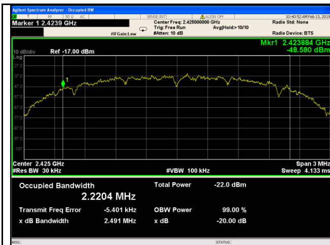
20dB Bandwidth – Low CH 2425
