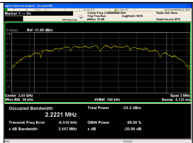
20dB Bandwidth - Middle CH 2450
