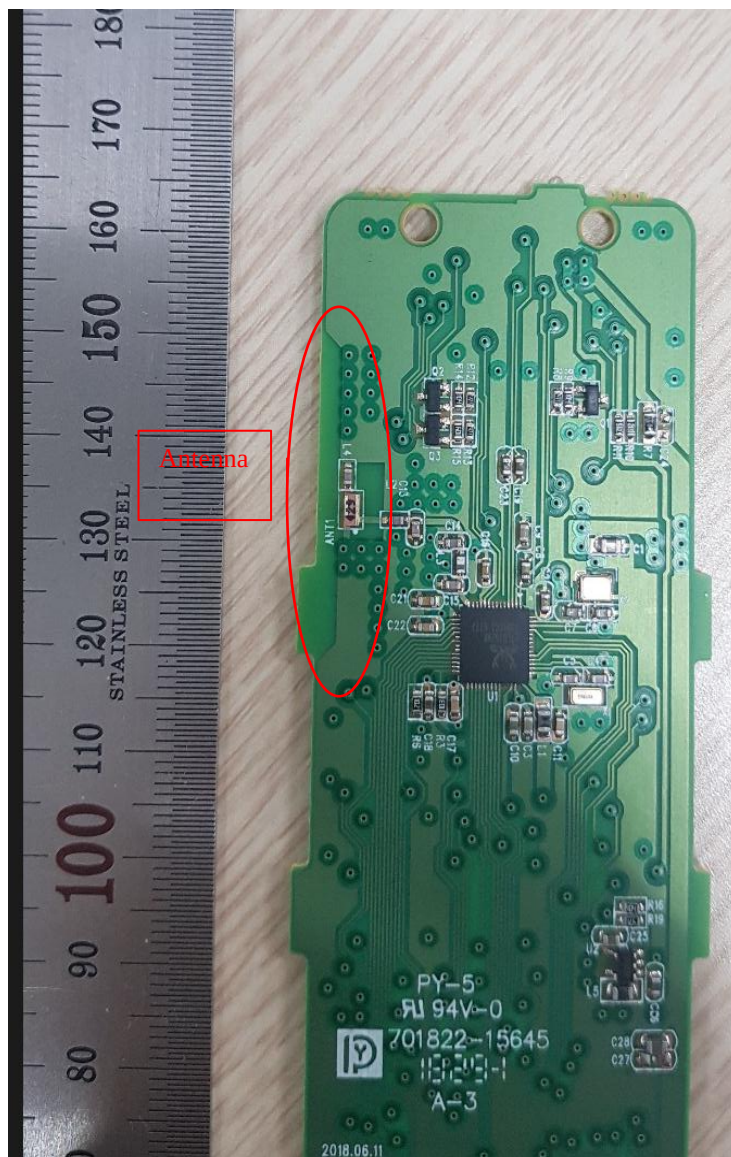
Antenna View
