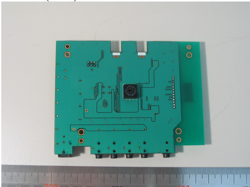
6. Bottom PCB View (RH55C)
