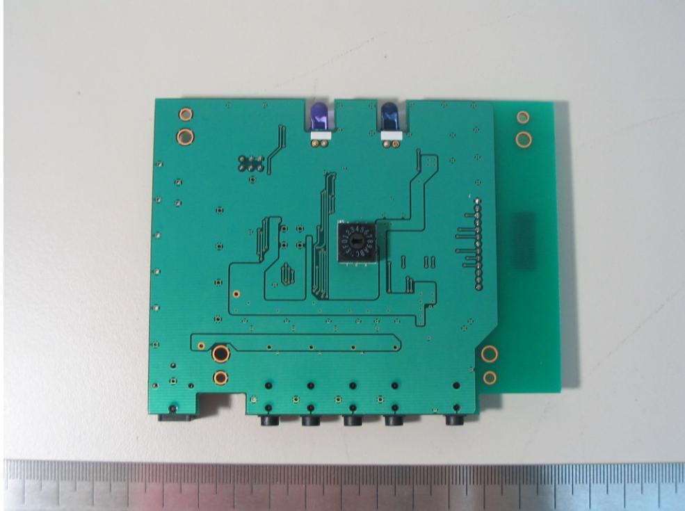
5. Bottom PCB View (RH55A)
