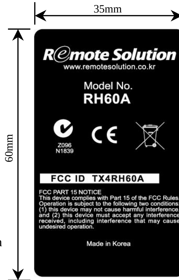
FCC Label main
