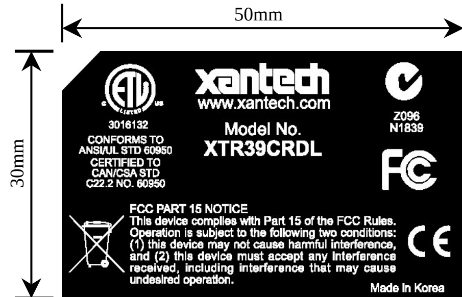
FCC Label Cradle
