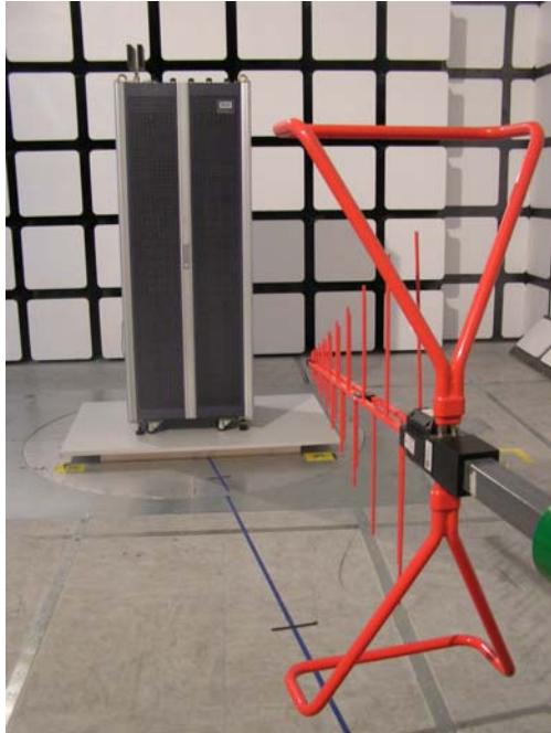
Radiated Emissions-Front View (below 1GHz)
