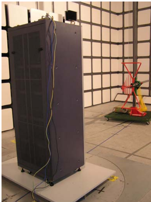
Radiated Emissions-Rear View (below 1GHz)
