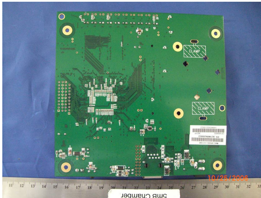
EUT – PCB1 Rear View
