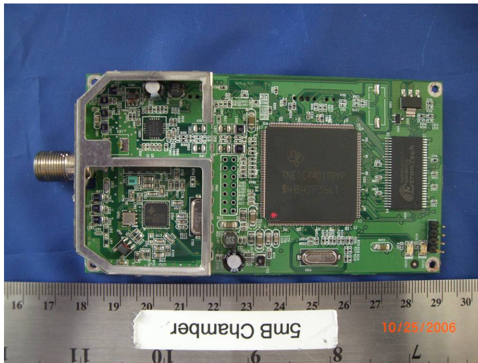
EUT - Sub board with Shield Off – Front View
