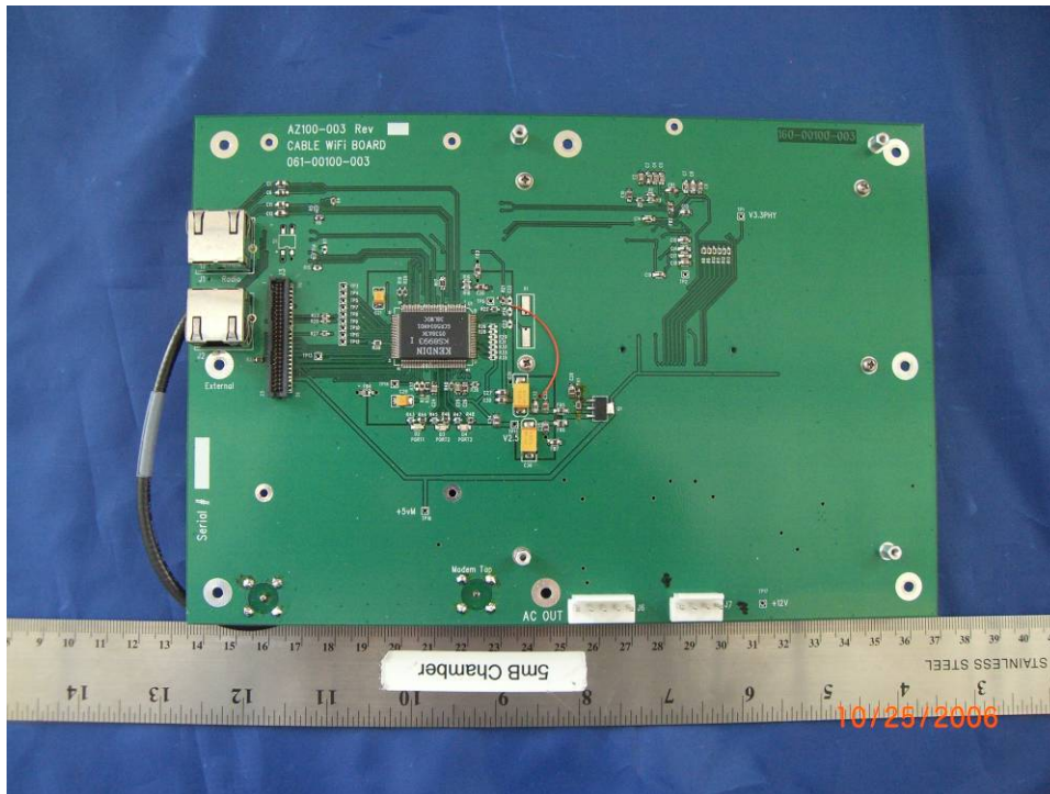
EUT - PCB2 - Back View
