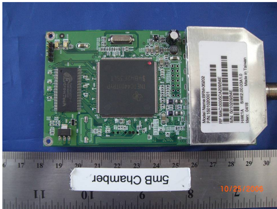
EUT - Sub Board with Shield on – Front View
