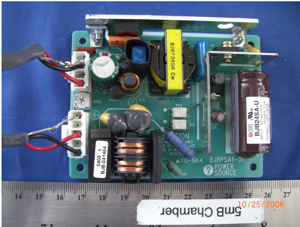
EUT - PCB3 – Back View
