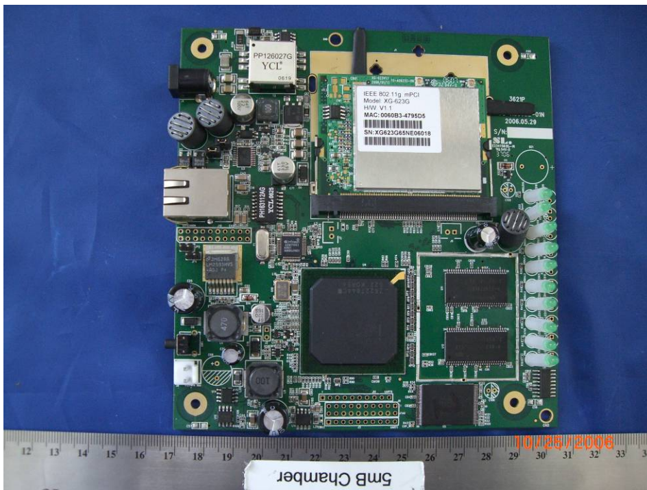
EUT – PCB1 with RF Board Front View
