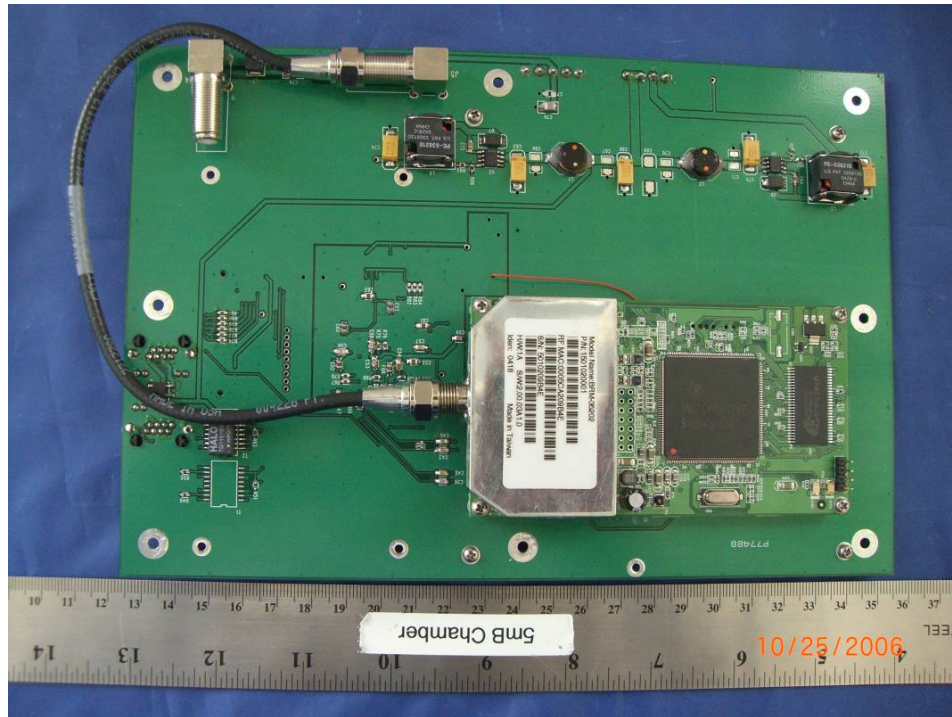
EUT - PCB2 with Sub Board - Front
