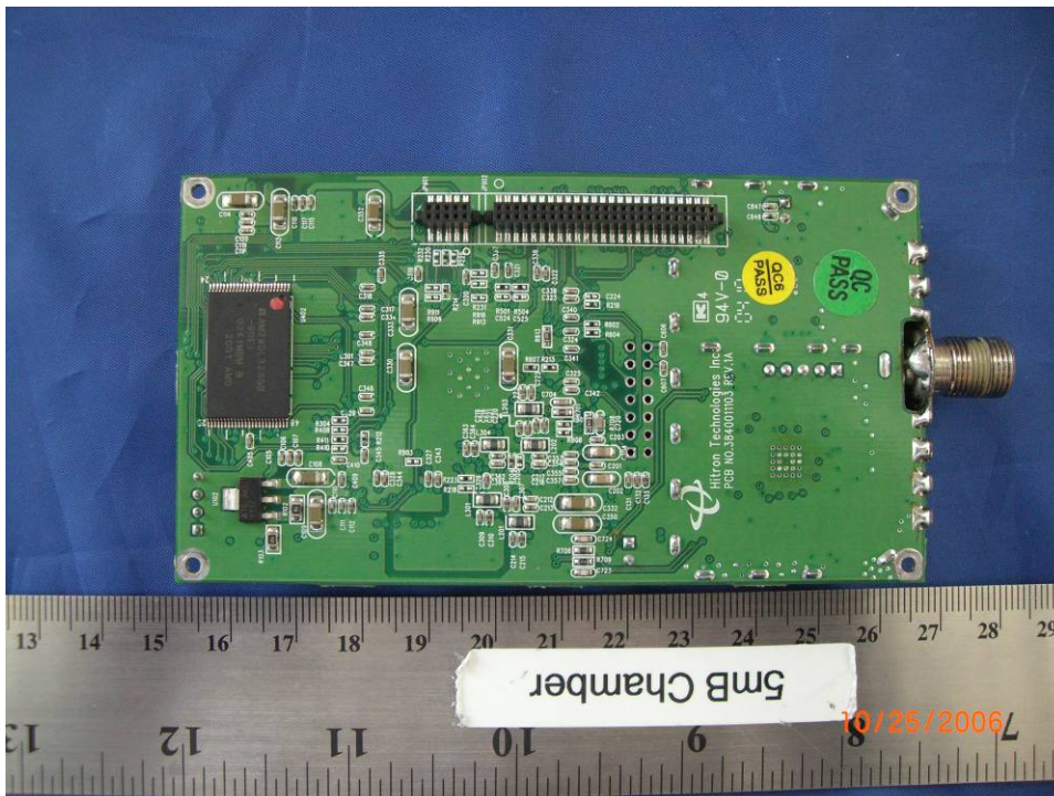
EUT - Sub Board - Back View
