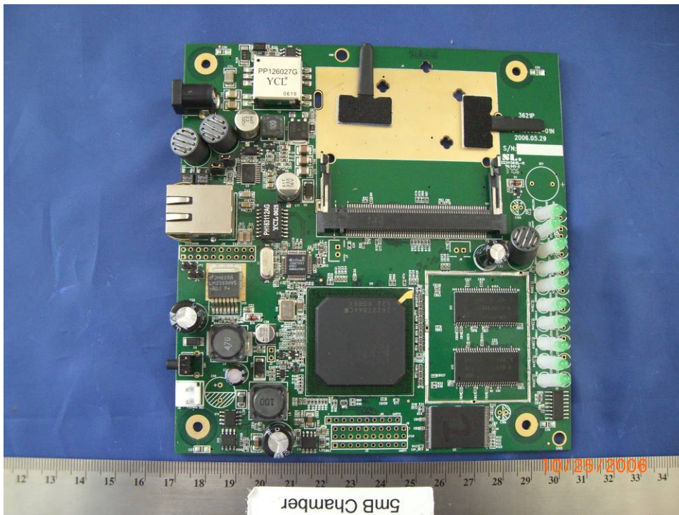
EUT - PCB1 without RF Board Front View
