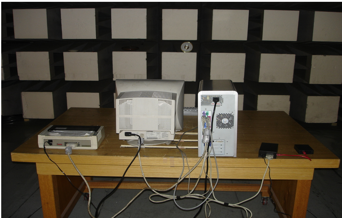
< Radiated emission – Rear >
