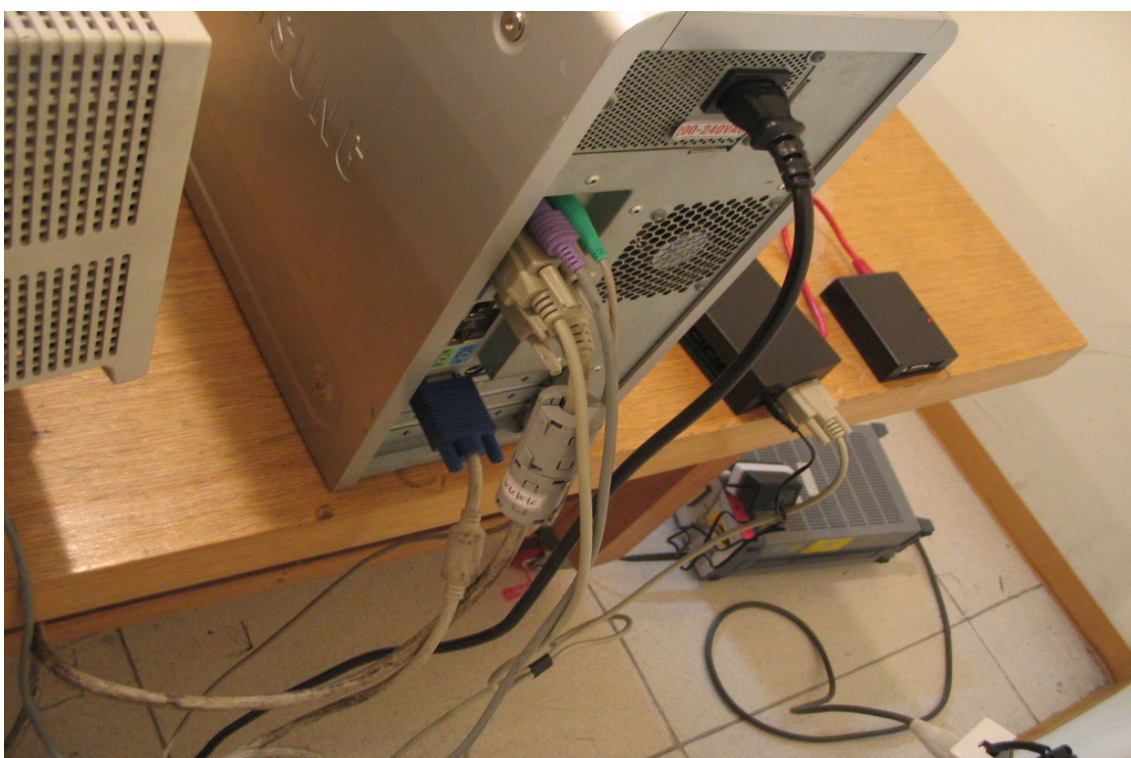
< Conducted emission – Rear >
