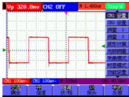
AC coupling
