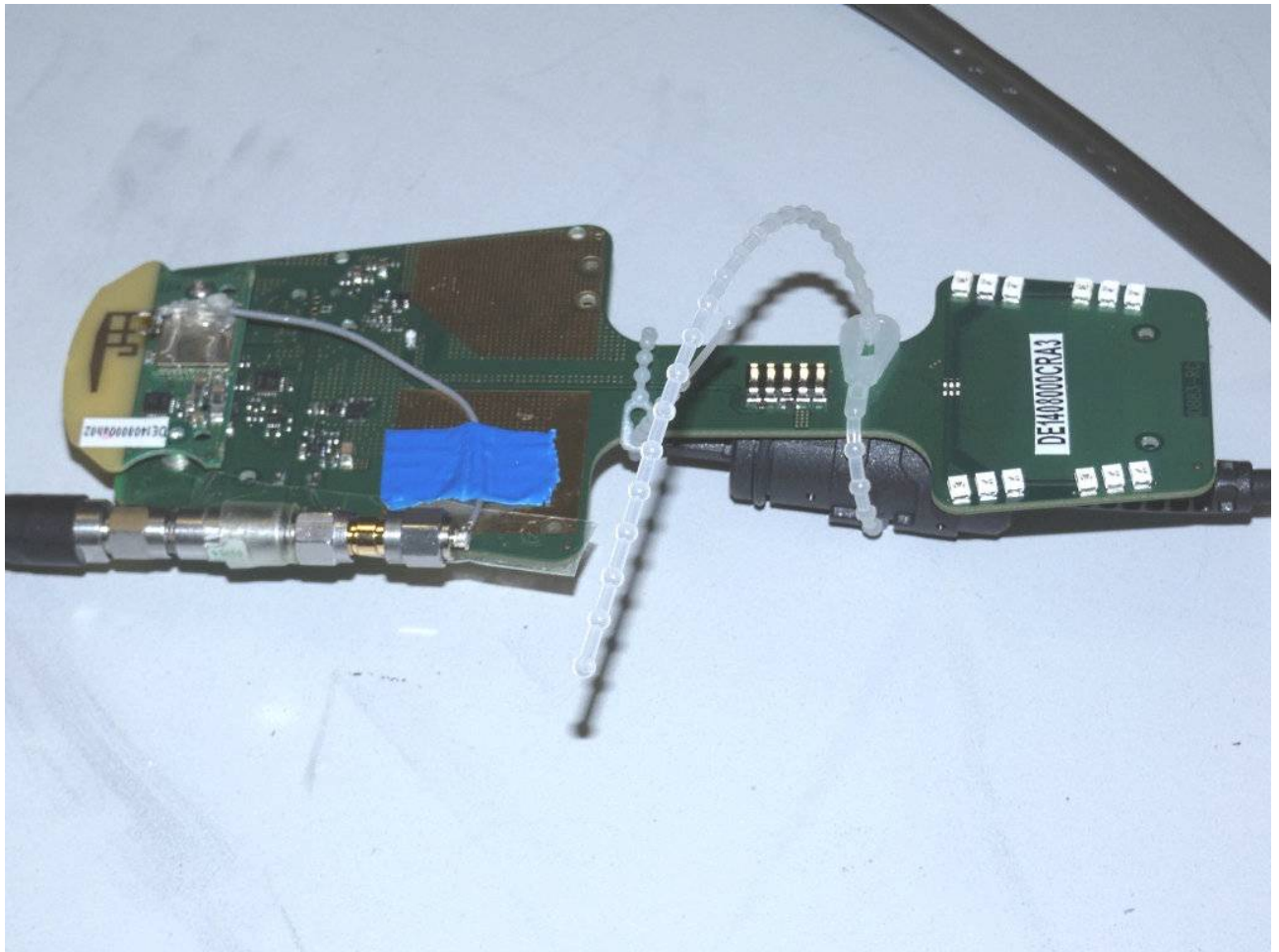
Photo 7: Test setup for conducted RF measurements (EUT in Cradle and temporary antenna connector, intentional radiator §15.247, ANSI C63.10)
