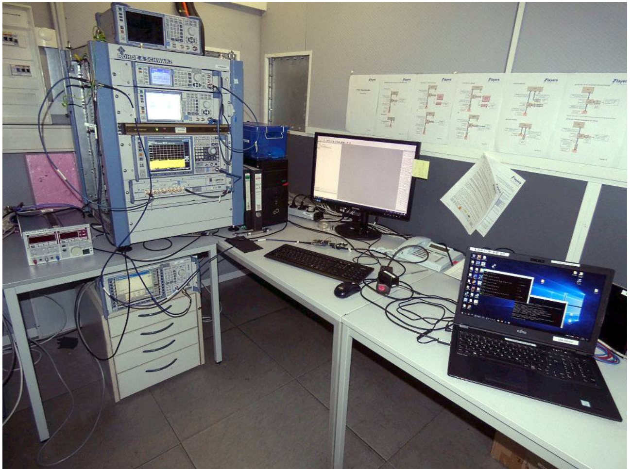
Photo 6: Test setup for conducted RF measurements (at temporary antenna connector using test system TS8997, intentional radiator §15.247, ANSI C63.10)
