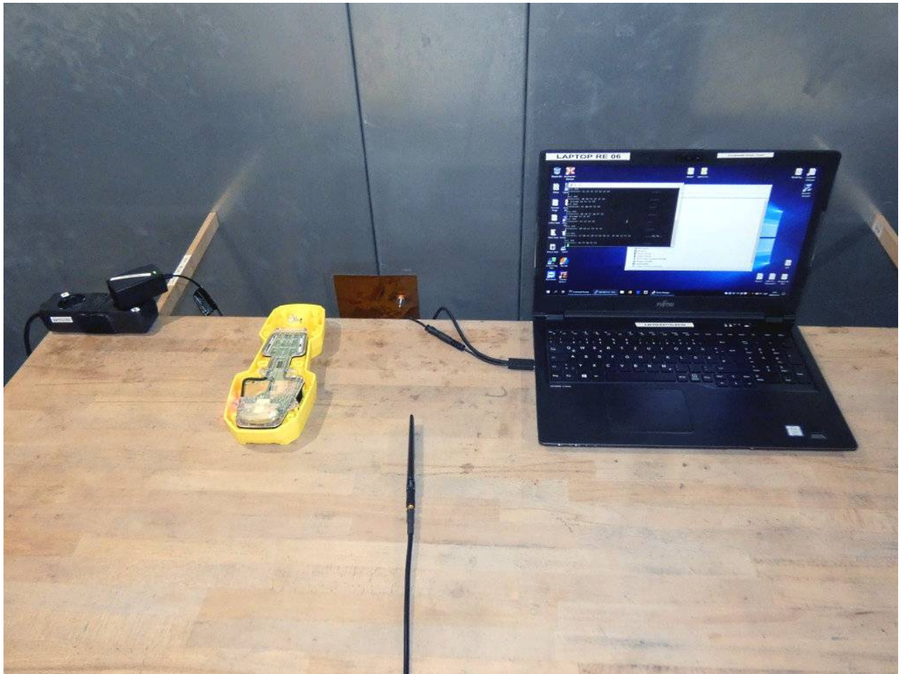
Photo 5: Test setup for conducted measurements (AC Port (power line), EUT supplied by AC/DC adapter, intentional radiator §15, ANSI C63.10)
