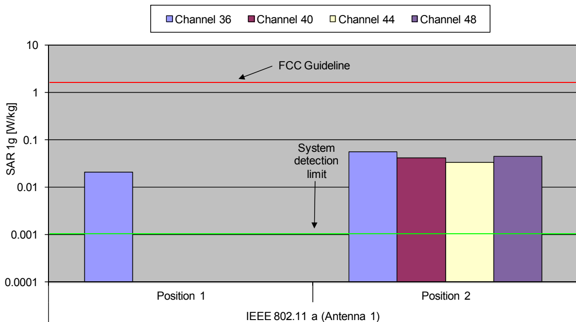
Fig. 9: The measured body SAR values for the Cognex DM9500 for IEEE 802.11 a in body worn configuration, in comparison to the FCC exposure limit.
