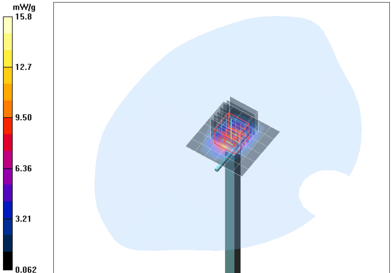
Fig. 10: Validation measurement 2450 MHz Body (September 21, 2012) coarse grid. Ambient Temperature: 22.0°C. Liquid Temperature: 21.9°C.
