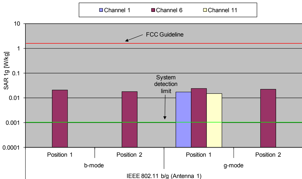
Fig. 8: The measured body SAR values for the Cognex DM9500 for IEEE 802.11 b/g in body worn configuration, in comparison to the FCC exposure limit.
