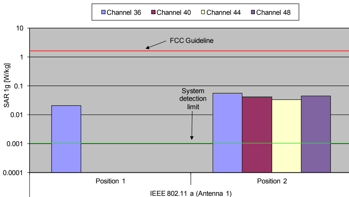
Fig. 9: The measured body SAR values for the Cognex DM9500 for IEEE 802.11 a in body worn configuration, in comparison to the FCC exposure limit.
