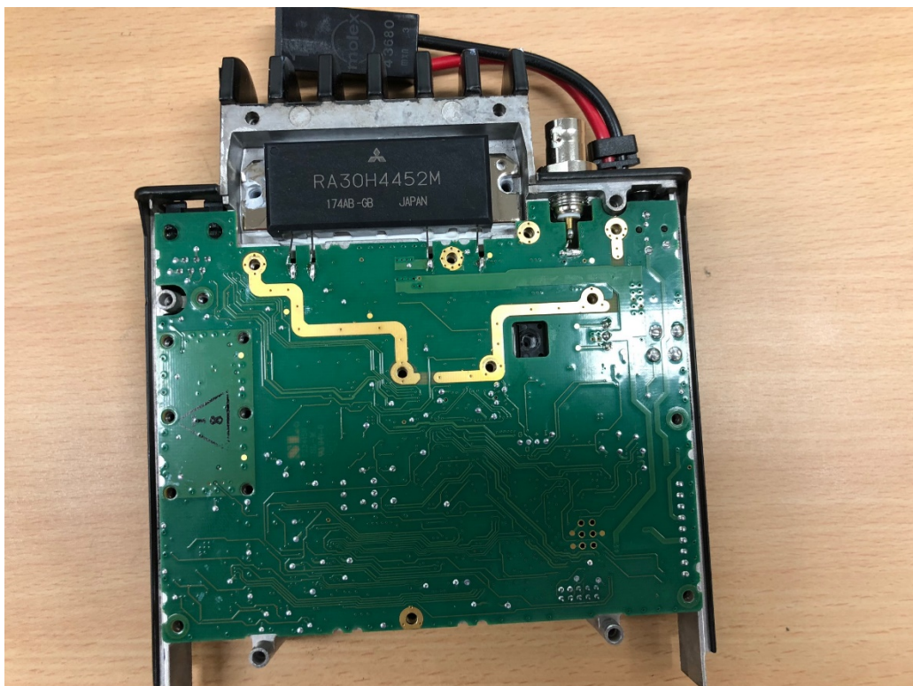
Bottom Main Board
